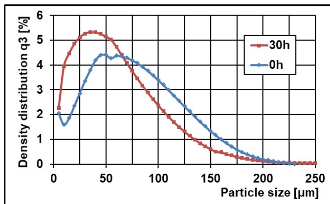
Fig. 3. Particle size distribution of the starting premixed powders and after milling for 30 hours
