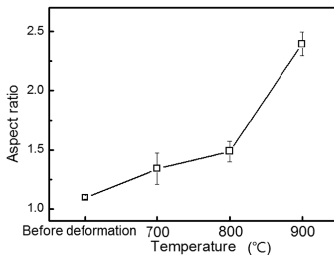
Fig. 4. Aspect ratio of the grains of Nd 12 Fe 82 B 6 with respect to deformation temperature
