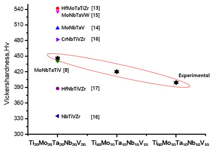
Fig. 3. Micro-Vickers hardness for TiMoTaNbV alloys homogenized at 1300^{\circ}C for 4 h. Vickers hardness values of the other refractory HEAs were referred for comparison
