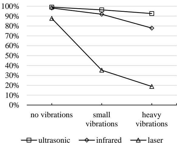
Fig. 6. Vibrations intensity influence on proximity sensors accuracy
