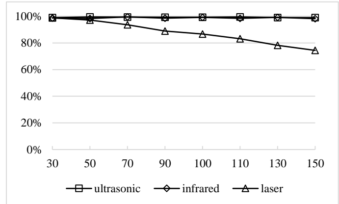
Fig. 3. Distance influence on proximity sensors accuracy
