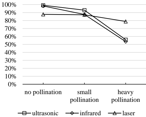
Fig. 5. Pollination intensity influence on proximity sensors accuracy
