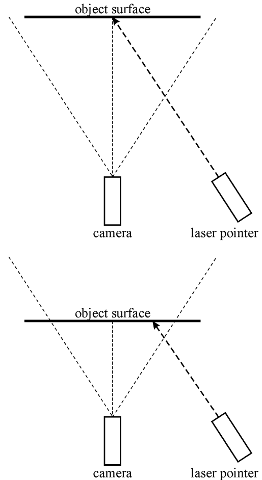
Fig. 1. Camera-to-object distance and laser dot coordinates
