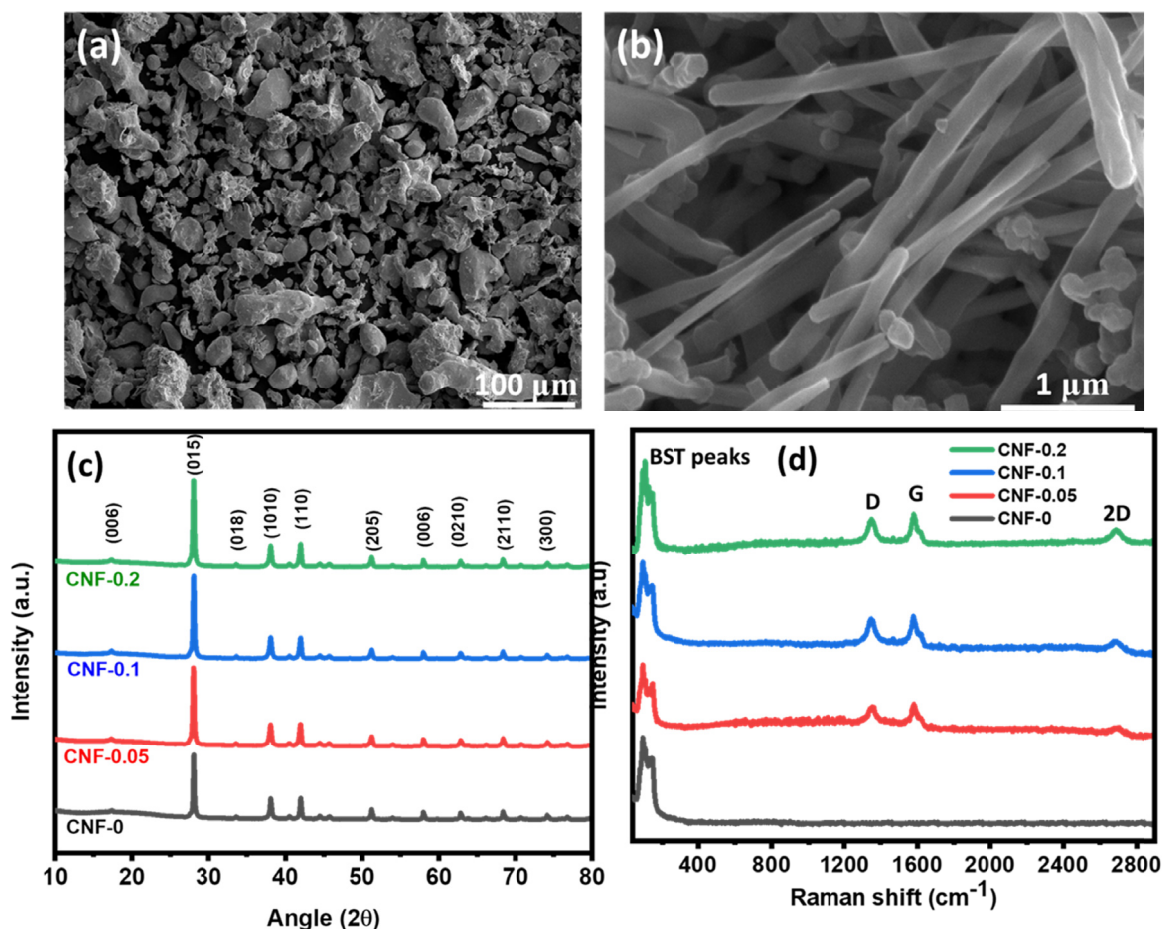
Fig. 1. The scanning electron microscope (SEM) images, (a) water atomized BST powder under 200 \mu\text{m} , (b) elongated carbon nanofiber as a dispersing material in BST matrix, (c) XRD peaks of BST/CNF bulk composites and their corresponding planes, and (d) room temperature Raman spectroscopy of bulk composites; lower and higher wavenumbers represents BST, CNF Raman spectral lines
