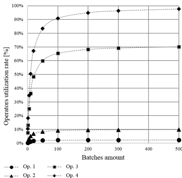
Fig. 6: Correlation between batch amount and operators utilization rate
