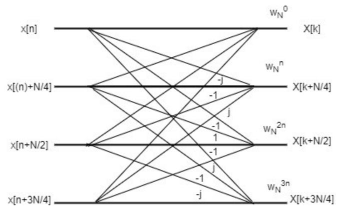
Fig. 1. Basic Radix-4 structure
