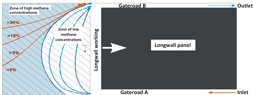
Fig. 1. Tendency of methane content distribution in the goaf of longwall ventilated by means of the “U” method
