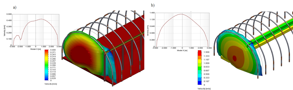
Fig. 20. Air velocity profile at the outlet from the Ventilation Drift (a) (Z-11 air roadway – Fig. 12) and the Maingate (b) (Z-11 roadway – Fig. 12) of longwall Z-11
