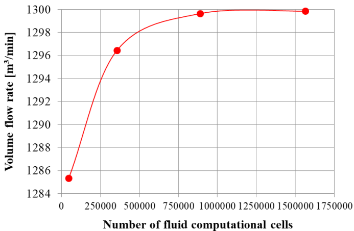
Fig. 8. Convergence of results in the numerical grid refinement study of longwall panel Z-11
