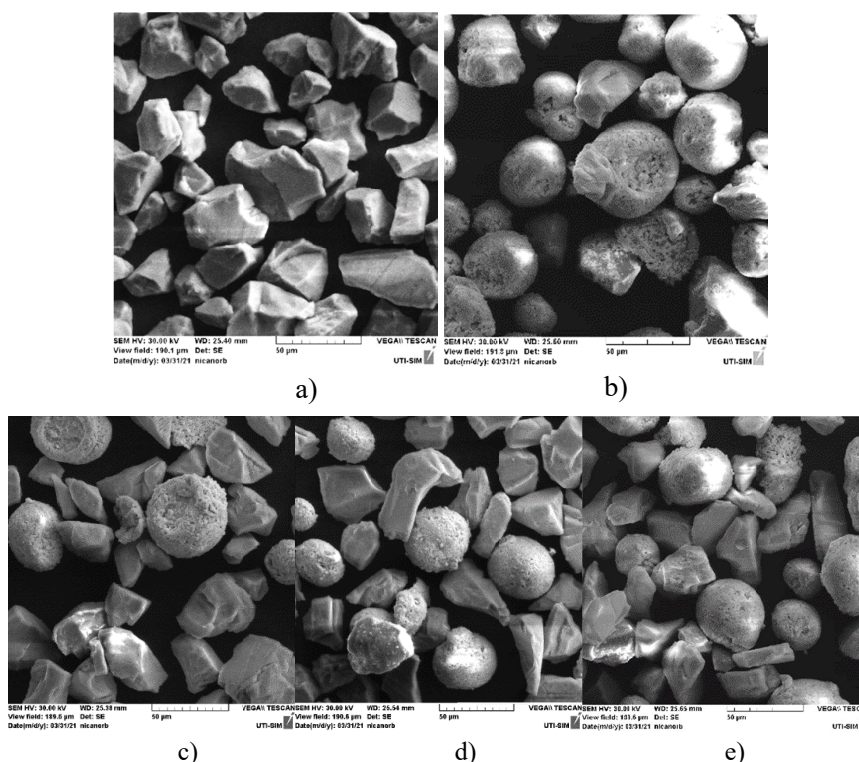
Fig. 1. SEM images of \text{Al}_2\text{O}_3 and \text{ZrO}_2 powders: \text{Al}_2\text{O}_3 in a) \text{ZrO}_2 in b), \text{Al}_2\text{O}_3+25\%\text{ZrO}_2 in c), \text{Al}_2\text{O}_3+50\%\text{ZrO}_2 in d) and \text{Al}_2\text{O}_3+75\%\text{ZrO}_2 in e)
