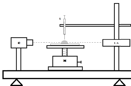
Fig. 2. Device used to measure the static contact angle
