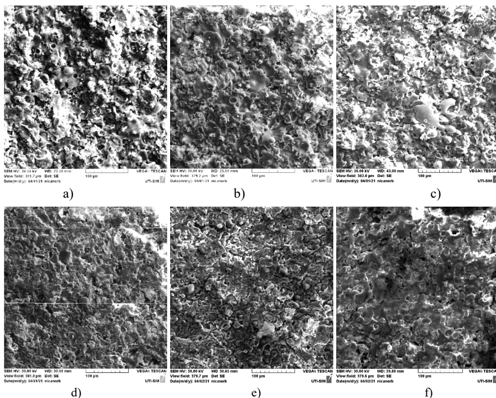
Fig. 3. SEM images of sample ceramic layers (a) \text{Al}_2\text{O}_3 -25% \text{ZrO}_2 , (b) \text{Al}_2\text{O}_3 -50% \text{ZrO}_2 and (c) \text{Al}_2\text{O}_3 -75% \text{ZrO}_2 and after mechanical grinding in d)-f)
