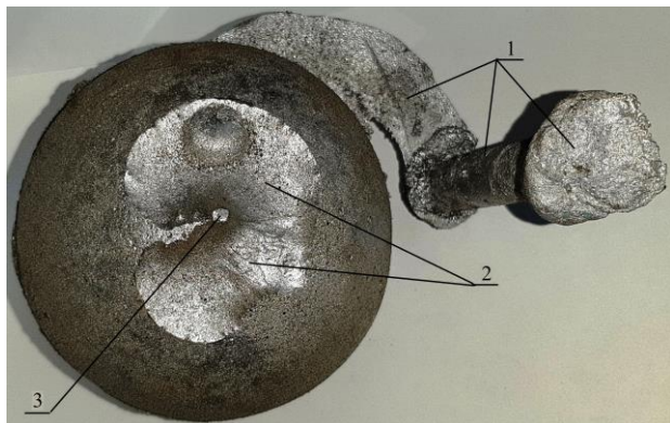
Fig. 7. Top view of the casting ball \varnothing 120 mm with the gating system (1), shrinkage depression (2) and remnant of an air gate (3)
