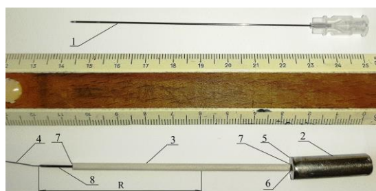
Fig. 3. Appliance for measurement vacuum in a shrinkage cavity: 1 - medical spinal needle \varnothing 0.7 mm x 90 mm; 2 - steel tube with the outer \varnothing 8 mm and wall thickness 1 mm; 3 - tube; 4 - wire \varnothing 0.2 mm; 5 - steel plug; 6 - zone of head welding 1 with steel cork; 7 - zone of sealing with ceramics gap between mullite silica tube 3 and head 1; 8 - part of the head without thermal insulation; R - depth of introduction into liquid metal, 60 mm
