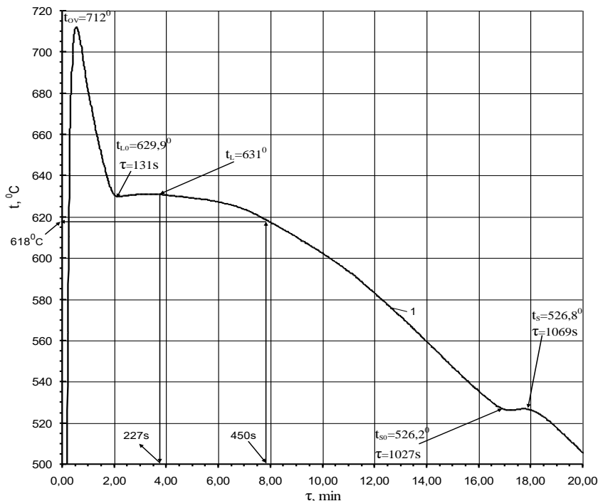
Fig. 6. Experimental cooling curve (1) of the centre of the sphere \varnothing 120 mm of Al-Si-Mg alloy in sand-and-clay casting mold: t_{L0} , t_L and t_{S0} , t_S - temperature of the beginning (o) and end of the temperature arrest at t_L and t_S , respectively; \tau - time
