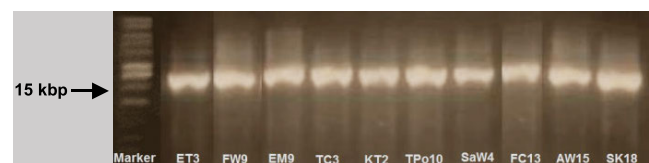
Fig. 1. Electrophoretic agarose-gel of the polymerase chain reaction (PCR) product after amplification of gene encoded the 16SrRNA (15 kbp of nucleotides) of rhizobacterial isolates; source: own study
