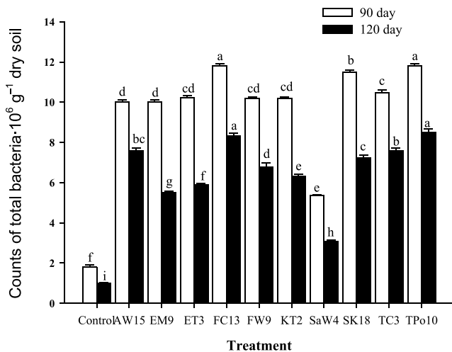
Fig. 2. Counts of total bacteria in the rhizosphere of wheat plants as affected by inoculation with plant growth-promoting rhizobacteria after 90 and 120 days from sowing date; error bars = mean standard error ( n = 3 ); the same letters in the Figure indicate no substantial difference at 0.05 significance level, determined by least significant difference (LSD) test ( n = 3 ); source: own study
