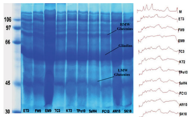
Fig. 4. Sodium dodecyl sulfate-polyacrylamide gel electrophoresis (SDS-PAGE) of proteins and its optical densities of bands at 660 nm extracted from grains of wheat cv. 'Sakha 94' as affected by rhizobacterial isolates; HMW = high molecular weight, LMW = low molecular weight; source: own study
