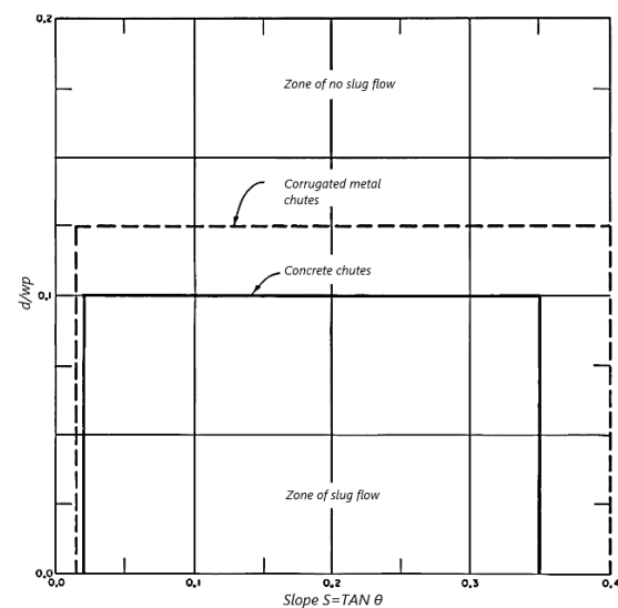
Fig. 4. Pulsating flow shape and criteria; d = average of water depth (m), \theta = angle of energy gradient, wp = wet perimeter; source: USBR [1987]
