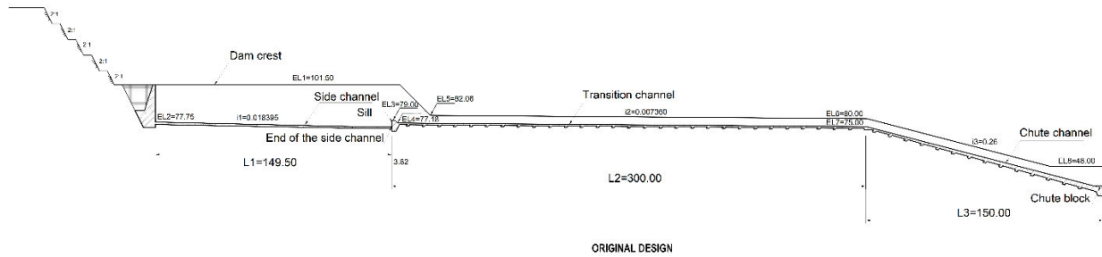
Fig. 2. Long profile of the experimental installation; source: own elaboration
