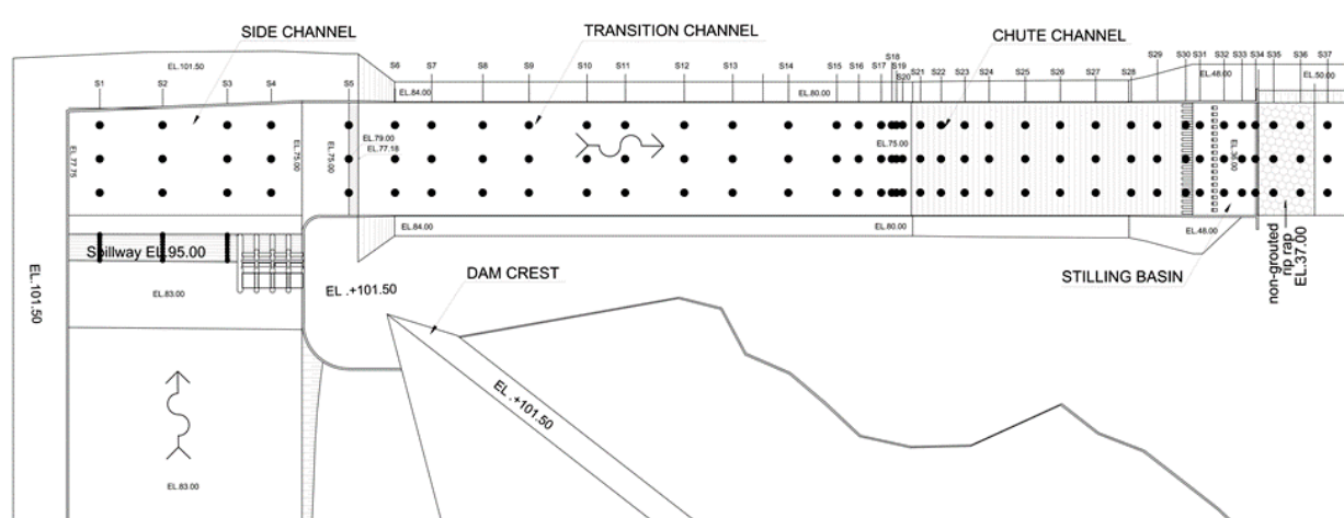
Fig. 1. Experimental installation and measurement points; source: own elaboration
