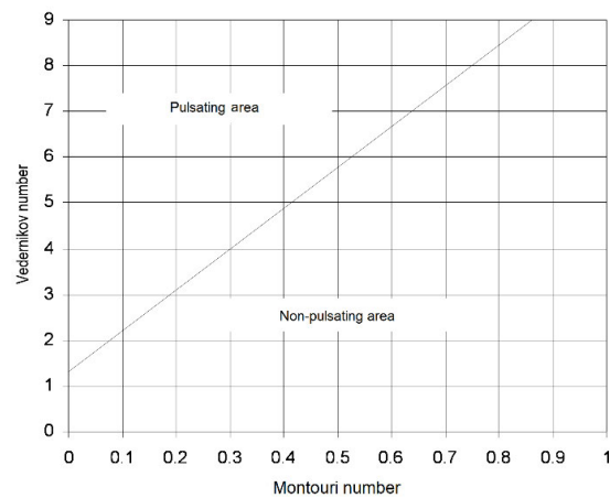
Fig. 3. Pulsating flow criteria graph; source: USBR [1987]
