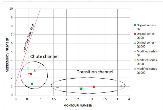
Fig. 7. Pulsating flow analysis in discharge variation for original and modified series; Q_2 , Q_{100} , Q_{1000} for original series as in Fig. 5 and modified series as in Fig. 6; source: own study
