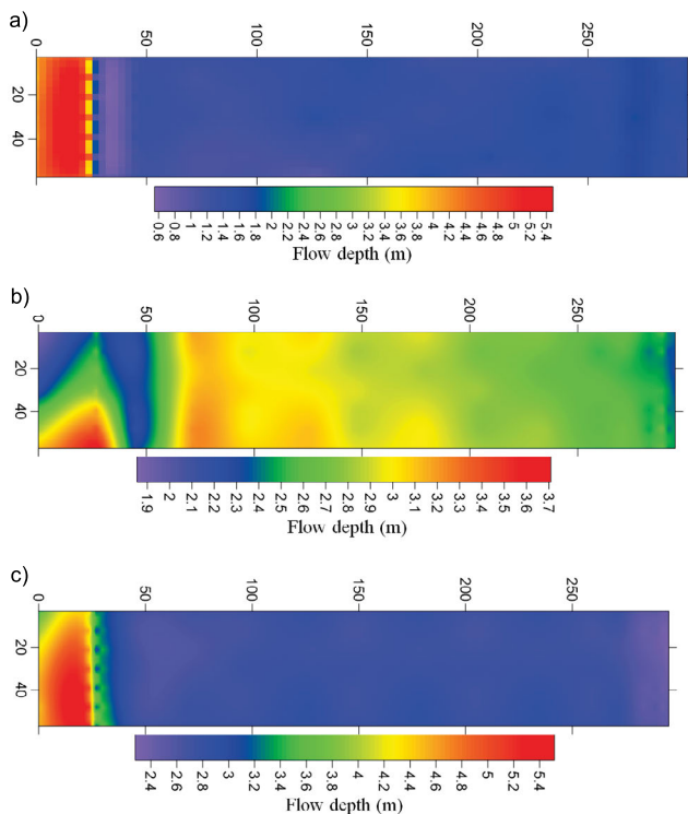
Fig. 6. Cross-waves after three physical model modifications (modified series): a) Q_2 = 5.72 \text{ m}^3 \cdot \text{s}^{-1} \cdot \text{m}^{-1} , b) Q_{100} = 16.62 \text{ m}^3 \cdot \text{s}^{-1} \cdot \text{m}^{-1} , c) Q_{1000} = 18.91 \text{ m}^3 \cdot \text{s}^{-1} \cdot \text{m}^{-1} ; source: own study
