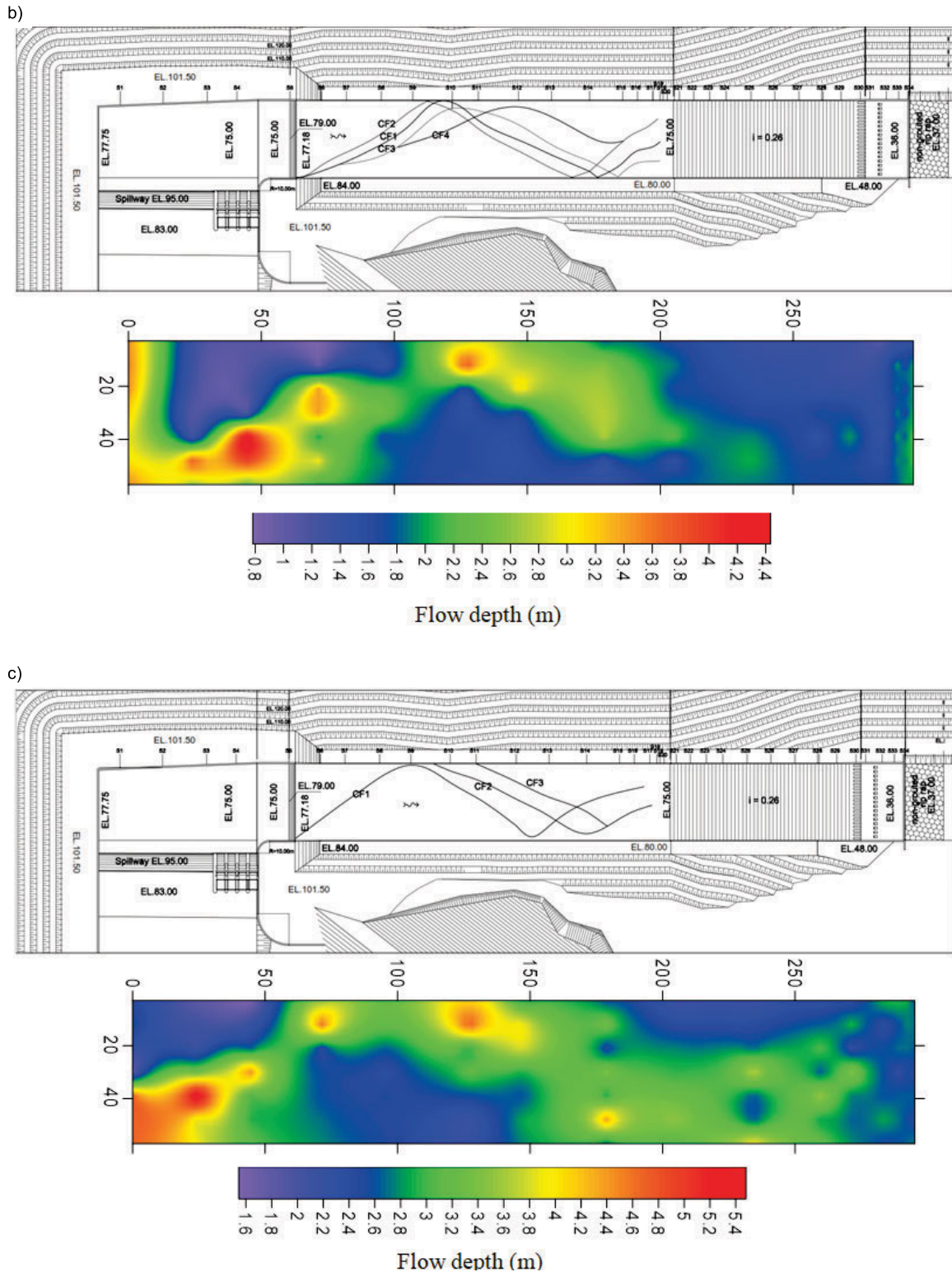
Fig. 5. Cross-waves at three different flow rates (original series): a) Q_2 = 5.72 \text{ m}^3 \cdot \text{s}^{-1} \cdot \text{m}^{-1} , b) Q_{100} = 16.62 \text{ m}^3 \cdot \text{s}^{-1} \cdot \text{m}^{-1} , c) Q_{1000} = 18.91 \text{ m}^3 \cdot \text{s}^{-1} \cdot \text{m}^{-1} ; source: own study
