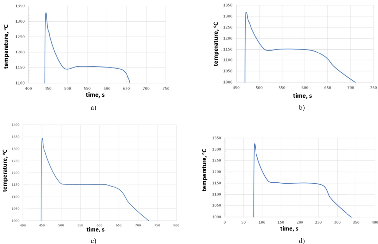
Fig. 10. Cooling and crystallization of inoculated grey cast iron for the melts: a) B1, b) B2, c) B3, d) B4
