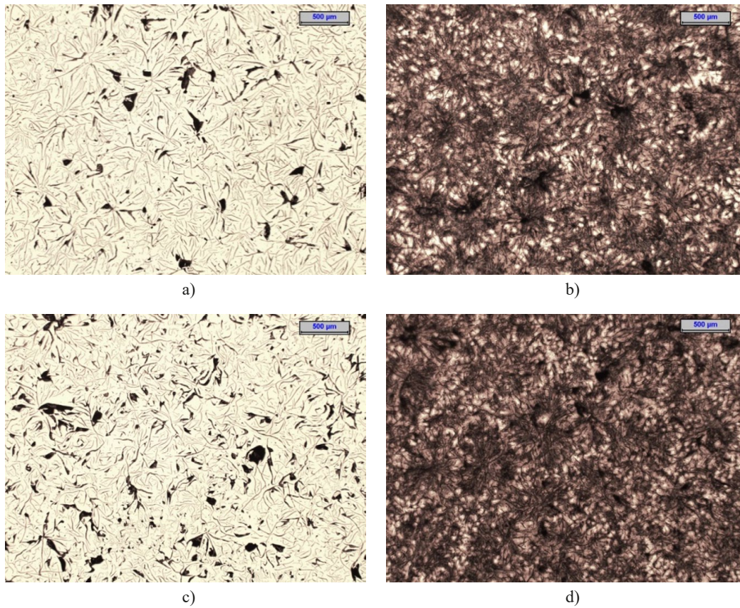
Fig. 13. Microstructure of cast iron (melt No 3B) after inoculation: „Y“-type ingot – a,b), roll casting with a diameter of Ø30 mm – c,d); nital etched – b,d) not etched – a,c)
