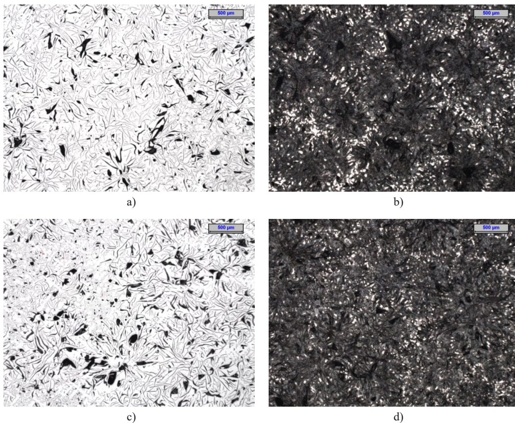
Fig. 14. Microstructure of cast iron (melt No 1B) after inoculation: „Y“-type ingot – a,b), roll casting with a diameter of Ø30 mm – c,d); nital etched – b,d) not etched – a,c)
