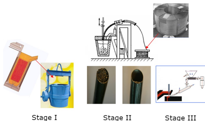
Fig. 8. Scheme of inoculation applied in Foundry Krakodlew S.A.: I – stage (when pouring from the furnace into the ladle), II – stage (introducing wire steel with and without a graphitizing inoculant using cored wire method), III – stage (on a stream of metal when pouring molds)
