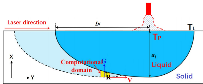
Fig. 1. Schematic of the laser molten pool in the macro-scale at early stage
