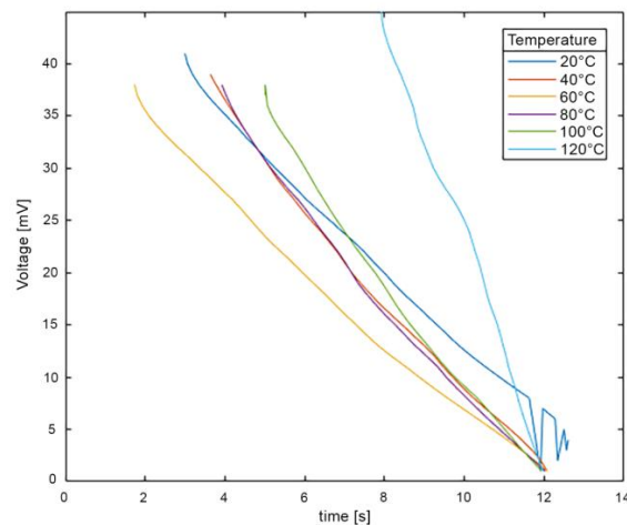
Fig. 5. Self-discharge curves (made out of measured points) for different values of temperature, the N_2 pressure being 122 kPa
