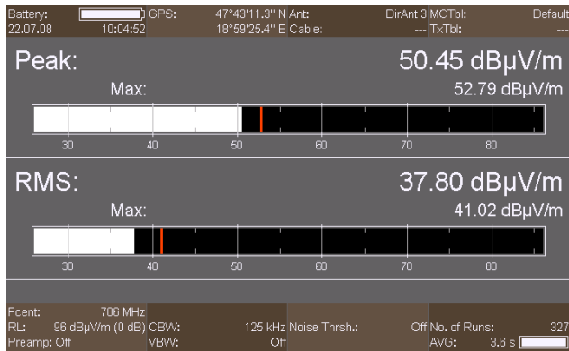
Fig. 6. Screenshot captured from the portable spectrum analyzer of the leakage values at 706 MHz
