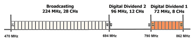
Fig. 1. Allocation of frequency channels in the UHF spectrum for ITU Region 1
