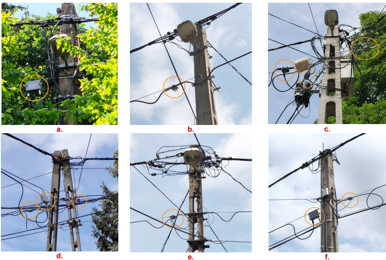
Fig. 7. Potential leakage sources of measurement samples; they are denoted by orange circles and are also listed in Table III
