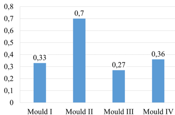
Fig. 6. Permeability of six-layered ceramic moulds
