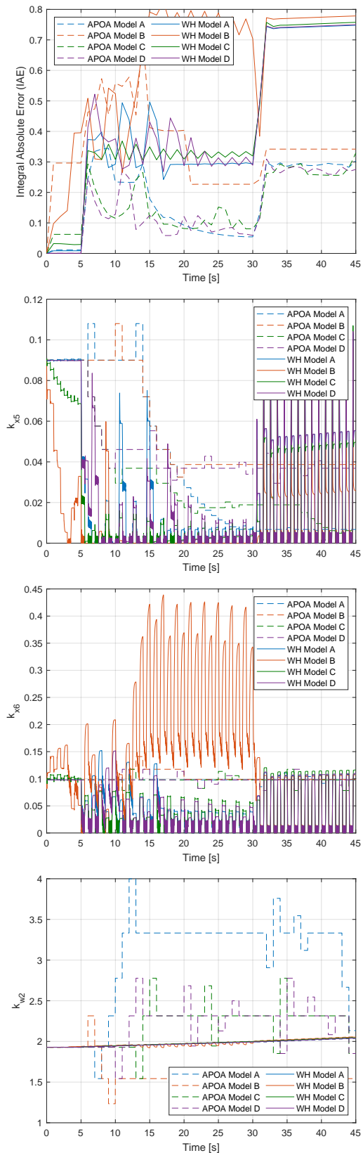
Fig. 7. Integral Absolute Error indicator and controller coefficients in time domain obtained for adaptation mechanism based on W-H rule and APOA with four difference model reference implementations. Operation under current limitation
