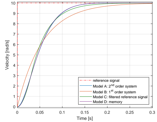
Fig. 3. Comparison of reference models
