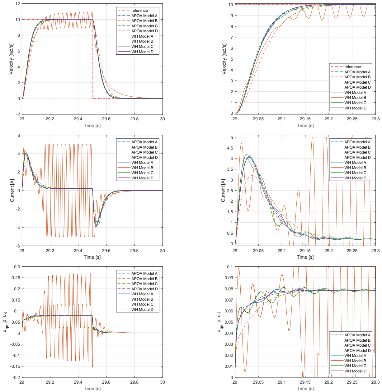
Fig. 5. Angular velocity, q -axis current, and q -axis control signal obtained for adaptation mechanism based on W-H rule and APOA with four different model reference implementations. Left column: entire signal reference period, right column: zoom in on the rising edge
