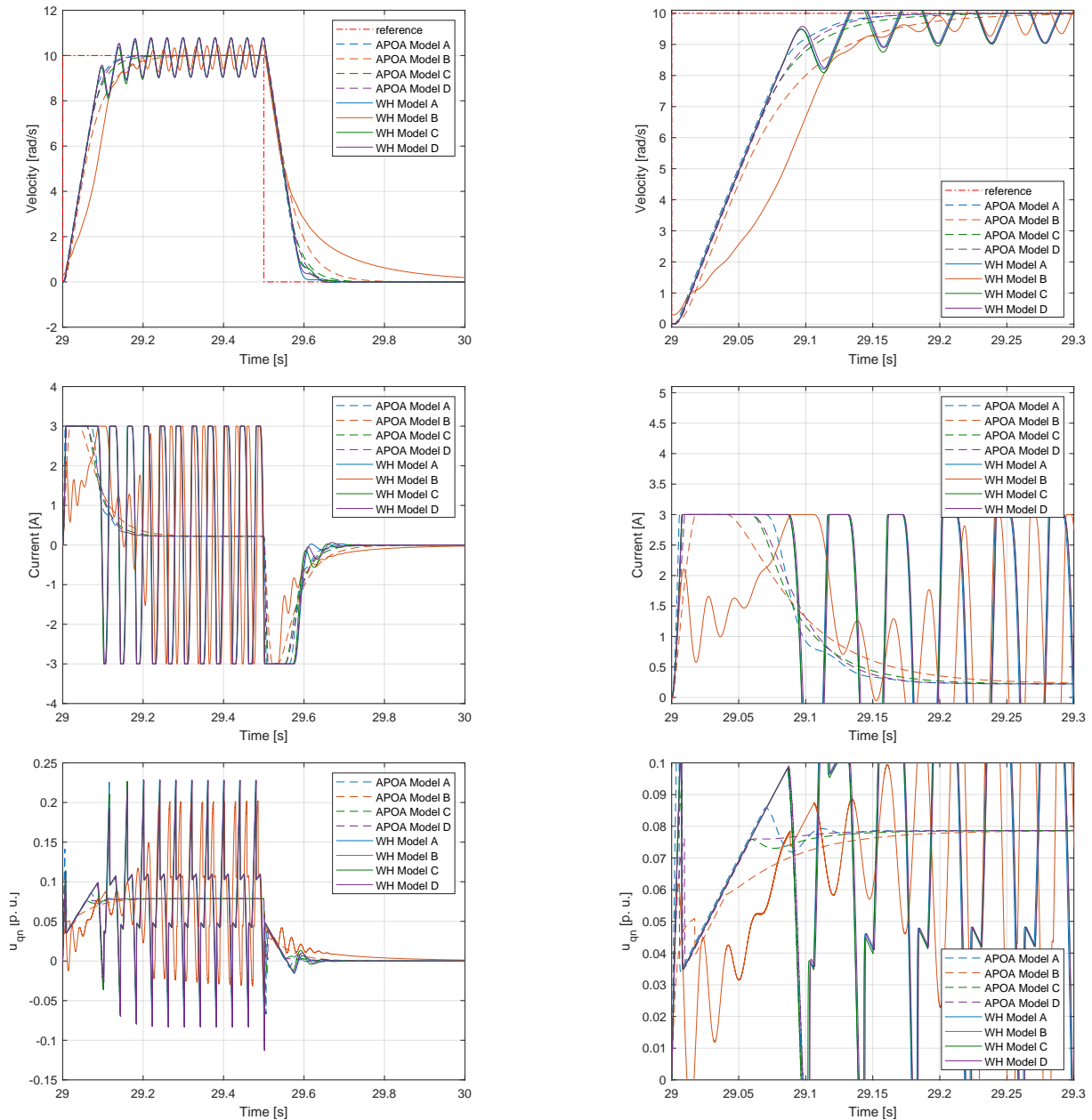
Fig. 8. Angular velocity, q -axis current, and q -axis control signal obtained for adaptation mechanism based on W-H rule and APOA with four different model reference implementations. Operation under current limitation to 3 A. Left column: entire signal reference period, right column: zoom in on the rising edge
