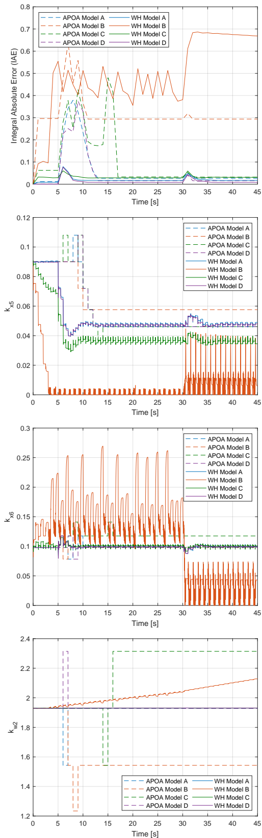
Fig. 6. Integral Absolute Error indicator and controller coefficients in time domain obtained for adaptation mechanism based on W-H rule and APOA with four difference model reference implementations
