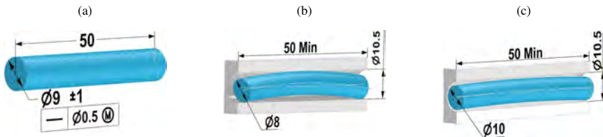
Fig. 18. (a) ASME specification – shaft diameter with the straightness tolerance of the axis; (b, c) interpretation – ring gauge of diameter 10.5 mm accepts smaller shafts with larger form deviations. [authors' drawing]
