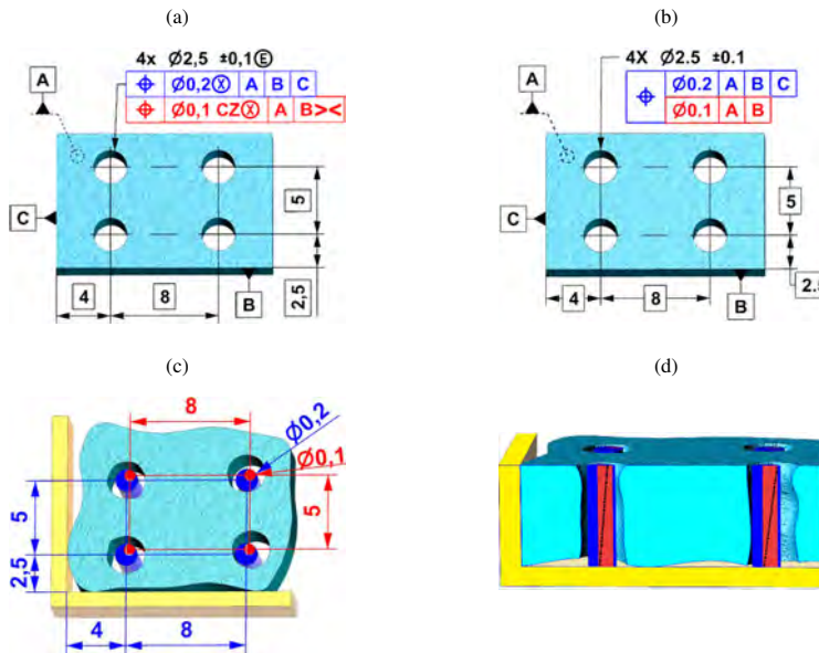
Fig. 26. Specification according to (a) ISO and (b) ASME; (c) visualisation of the tolerance zones according to ISO and ASME – top view; (d) interpretation – axis of the cylinder inscribed in each actual hole shall be within the respective cylindrical tolerance zones of diameters 0.2 mm and 0.1 mm. [authors' drawing]
