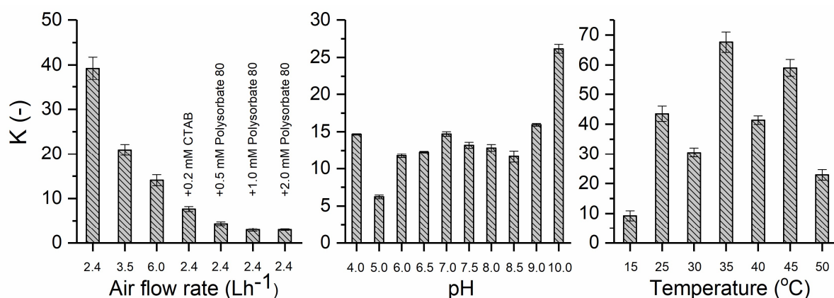
Figure 4. The partitioning coefficient of all tested systems in the process of foam fractionation.
