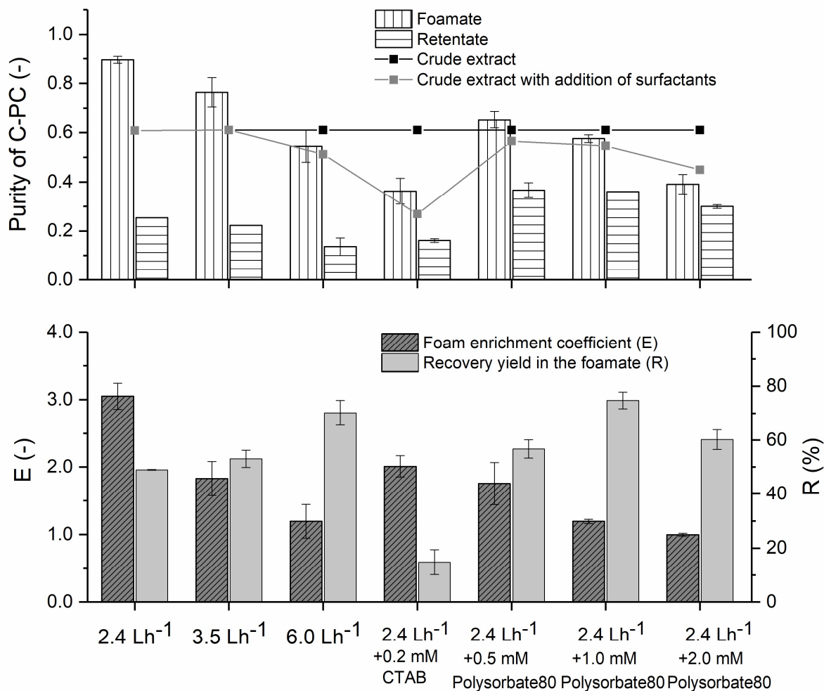
Figure 1. The purity of C-PC in foamate and retentate after FF process and in crude extract with and without the addition of surfactants (above); the enrichment coefficient and recovery yield in the foamates (below) in the systems with different values of air flow rates and with the addition of surfactants.
