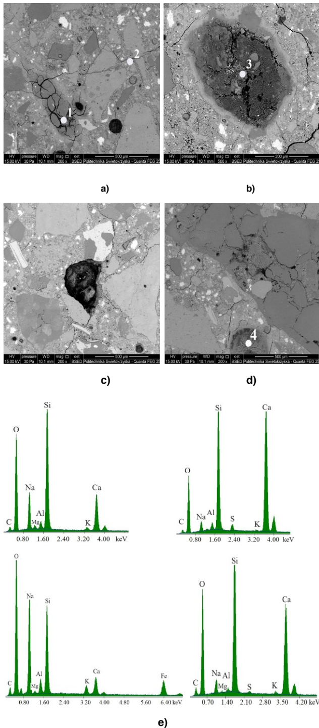
Fig.5. Microstructure images of the mortar depicting: a-b) cracked reactive aggregate grains, c) aggregate relic, d) air void filled with ASR, e) X-ray microanalysis at points 1-4.
