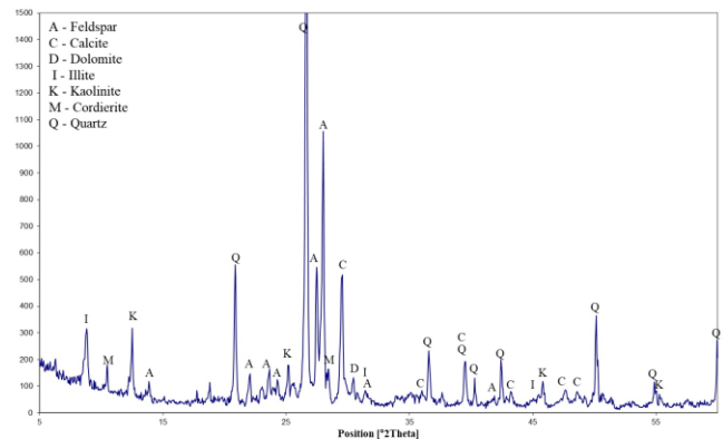
Fig.1. XRD diffraction pattern of gravel aggregate [17]
