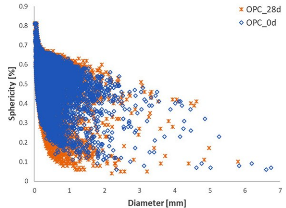
Fig.4. Dependence of pore sphericity on diameter in mortars after 0 and 28 days of the test
