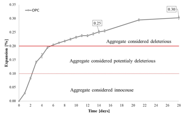
Fig.2. Expansion behavior of the mortar bars containing mechanically crushed gravel aggregate
