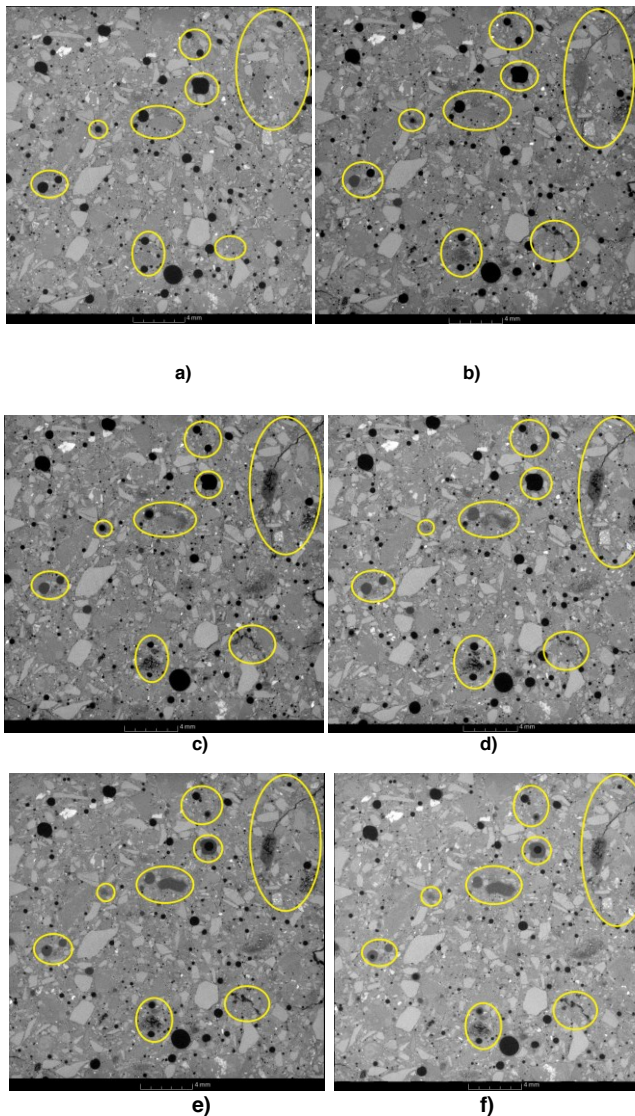
Fig.3. 2D images obtained by X- ray \mu CT of gravel aggregate mortars stored in 1M NaOH after: a) 0 days, b) 3 days, c) 7 days, d) 14 days, e) 21 days, f) 28 days. Corrosion centers and air voids gradually filled with gel were marked in yellow.
