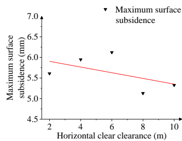
(c) Horizontal clear clearance
