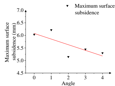
(d) The angle between the tunnel axis and karst cave axis
