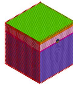
(b) Boundary constraint condition
