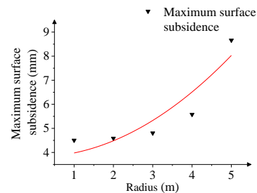
Fig.4. The relationship between radius and maximum surface subsidence
