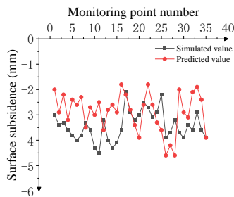
Fig.1. Comparative map of surface subsidence
