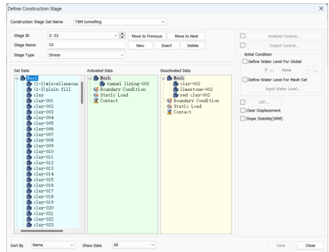
(c) Define construction stage
