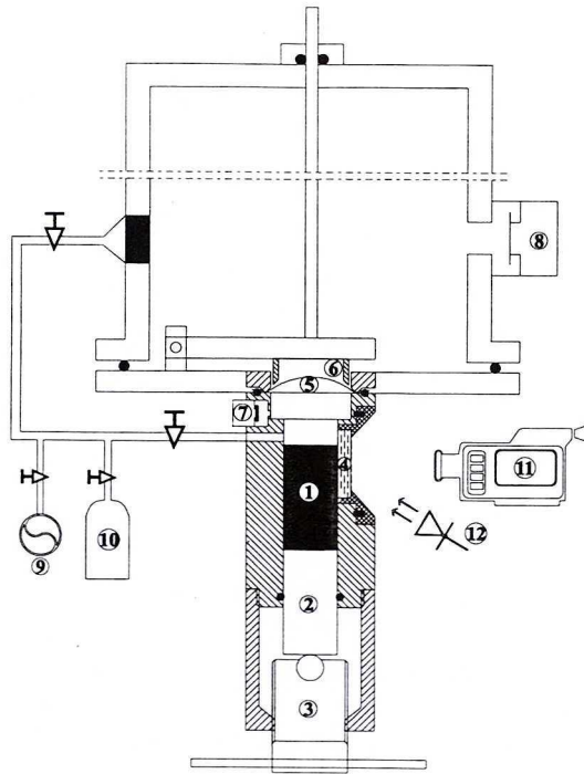
Fig. 3. Experimental setup for recording the coal briquette destruction
