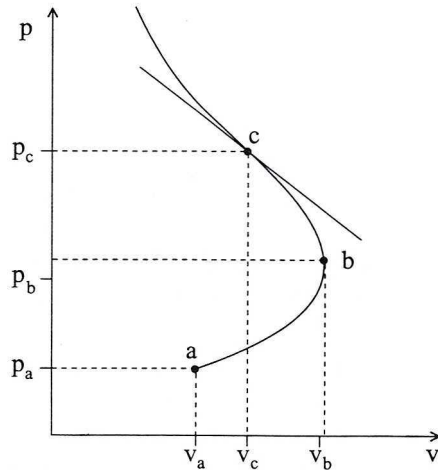
Fig. 1. The pressure p vs specific volume V for coal samples saturated with gas
