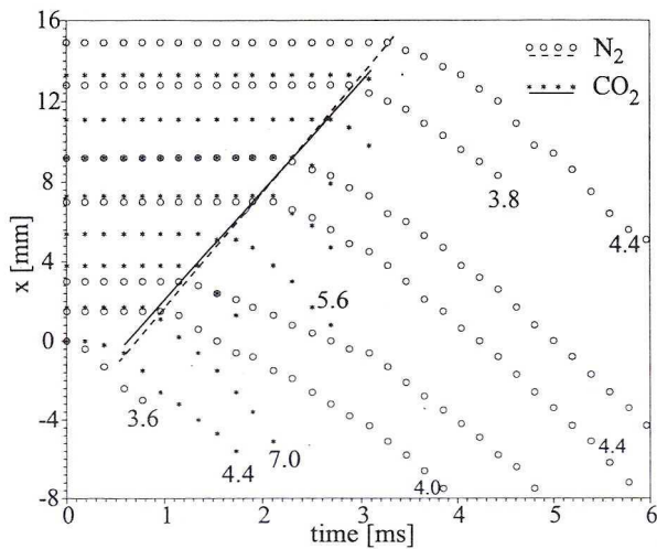
Fig. 5. A slices movement during briquette destruction (on the ground of Fig. 4)
