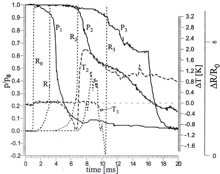
Fig. 9. Pressure, deformations and temperature — a briquette saturated with He
