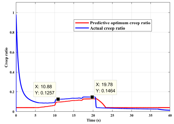
Fig. 15. Creep ratio performance based on torque correction method
