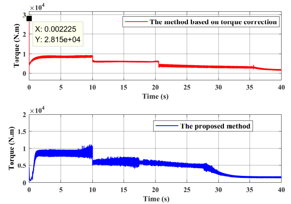
Fig. 20. IPMSM output torque performance in the HIL platform
