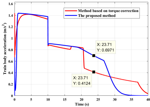
Fig. 13. Performance of train body acceleration with comparative simulation
