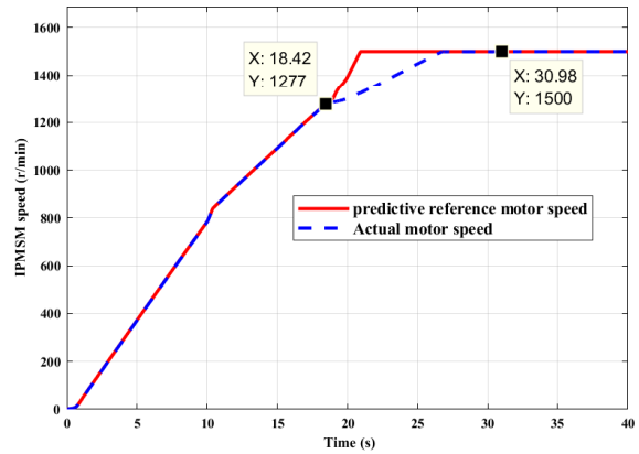
Fig. 9. IPMSM speed tracking performance
