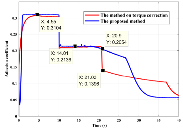
Fig. 14. Performance of train adhesion coefficient with comparative simulation
