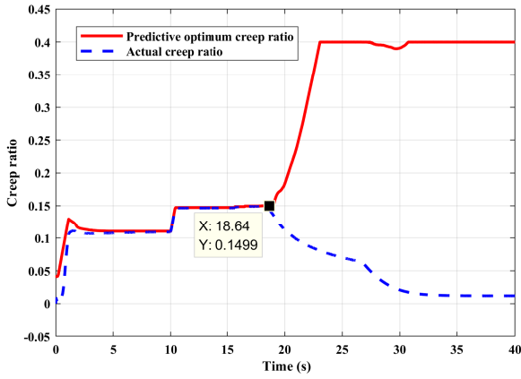
Fig. 11. Creep ratio performance
