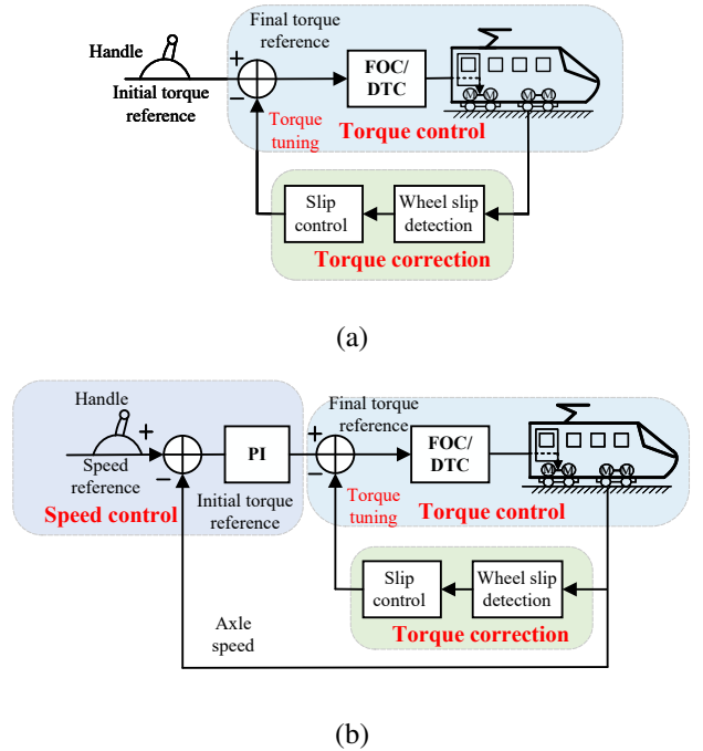
Fig. 1. Block diagram of a conventional torque correction-based adhesion control strategy : (a) Manual mode; (b) Automatic mode.
