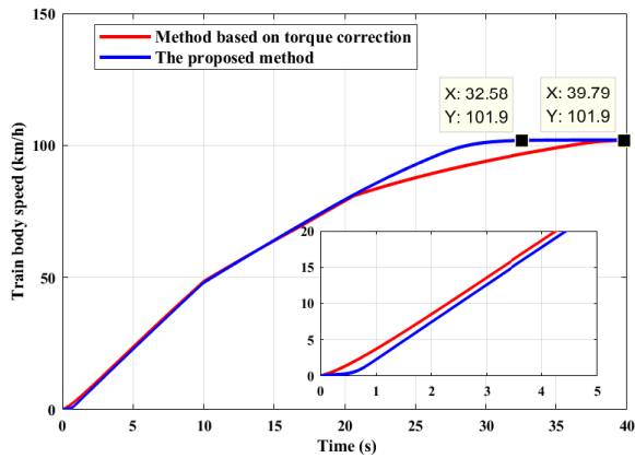
Fig. 12. Performance of train body speed with comparative simulation
