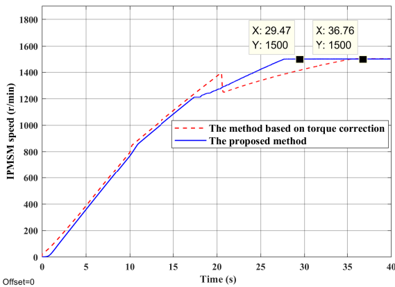
Fig. 18. IPMSM speed tracking performance in the HIL platform
