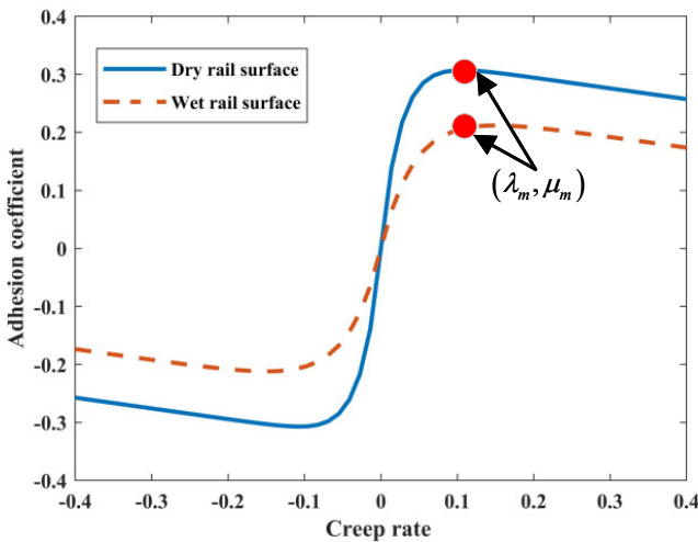
Fig. 3. Adhesion characteristics curve
