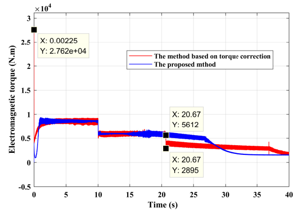
Fig. 16. IPMSM electromagnetic torque performance with comparative simulation
