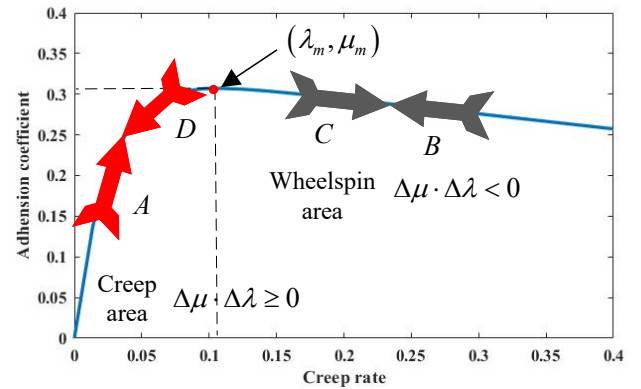
Fig. 5. Classification diagram of each operation point on the adhesion curve
