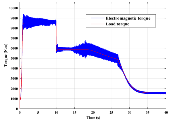
Fig. 10. IPMSM electromagnetic torque and load torque performance
