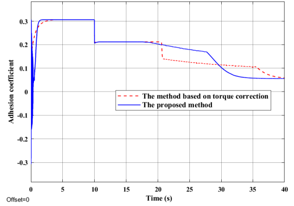
Fig. 19. Adhesion coefficient tracking performance in the HIL platform
