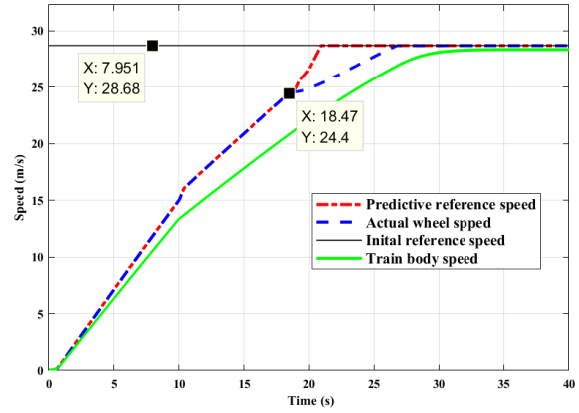
Fig. 8. Wheel and train body speed tracking performance
