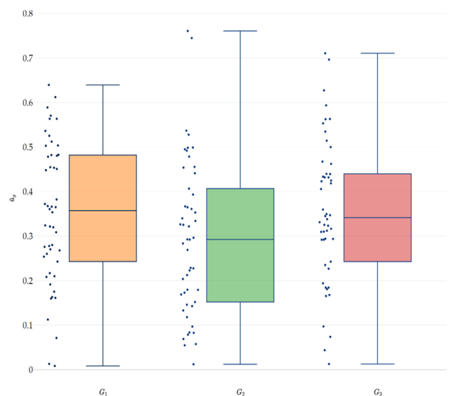
Fig.11. Statistics of generated weights for the group of main criteria G_1 - G_3
