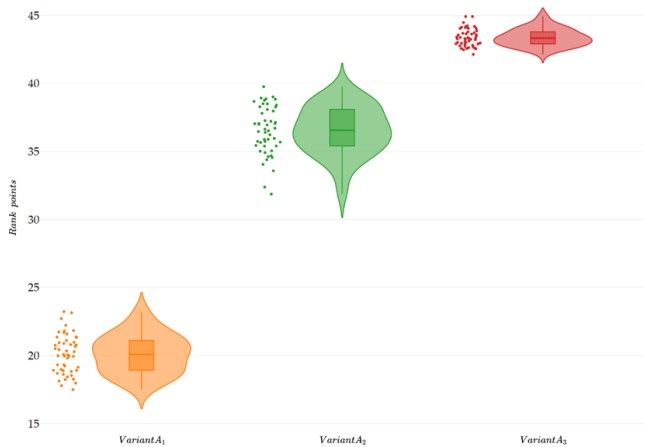
Fig.12. Distribution of points obtained in the rankings of the FAHP method for individual alternatives obtained for 50 iterations of random weight \tilde{u}_g .
