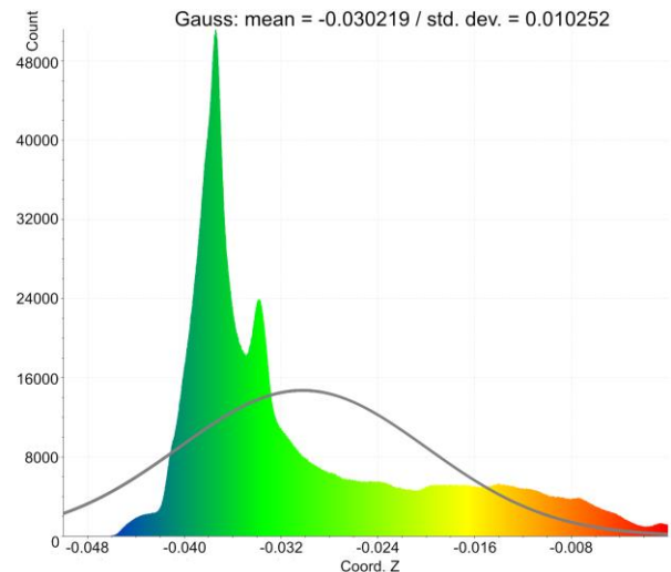
Fig.7. Histogram of floor plate deflections
