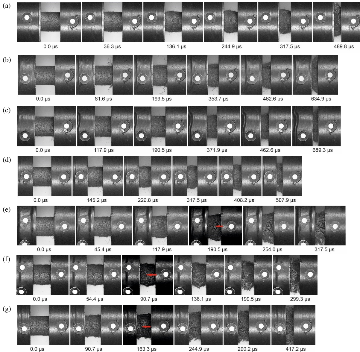
Fig. 7. Frames taken from video records of DIHPB tests of: (a) Ti+100AC; (b) Ti64BEPM+50AC; (c) Ti64BEPM+75AC; (d) Ti64BEPM+100AC; (e) Ti64PA+50AC; (f) Ti64PA+75AC; (g) Ti64PA+100AC (Red arrows in (e, f, g) indicates appearance of brittle cracks)
