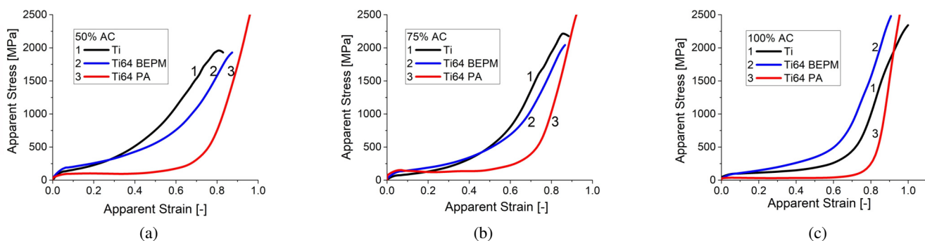
Fig. 9. Comparison of dynamic compression curves for porous Ti (curves 1) and Ti64 (2, and 3) prepared by two different ways (2 – BEPM method, 3 – using pre-alloyed powder) depending on amount of space holder (ammonium carbonate – AC): (a) 50%, (b) 75%, (c) 100%. Data for porous Ti obtained with additions of 50% and 75% ammonium carbonate in (a) and (b) were taken from previous work [12]
