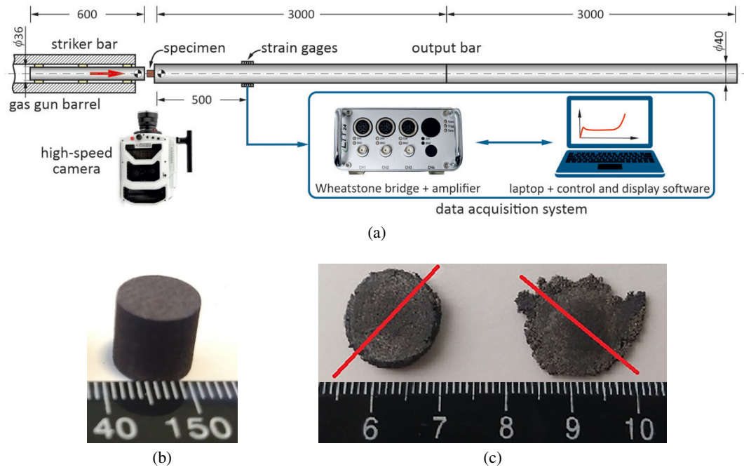
Fig. 2. Scheme of the SHPB apparatus used for dynamic strength tests [12] (a), general view of the samples before (b) and after the DIHPB tests (c) – the red lines represent the planes along which the tested samples were cut for fractographic and metallographic examinations
