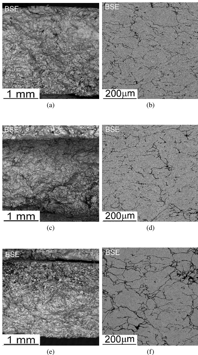
Fig. 12. Fracture surfaces (a, c, e) and microstructure (b, d, f) of porous Ti64PA samples after DIHPB tests. Amount of AC in the initial mixture: (a, b) 50%; (c, d) 75%; (e, f) 100%. SEM
