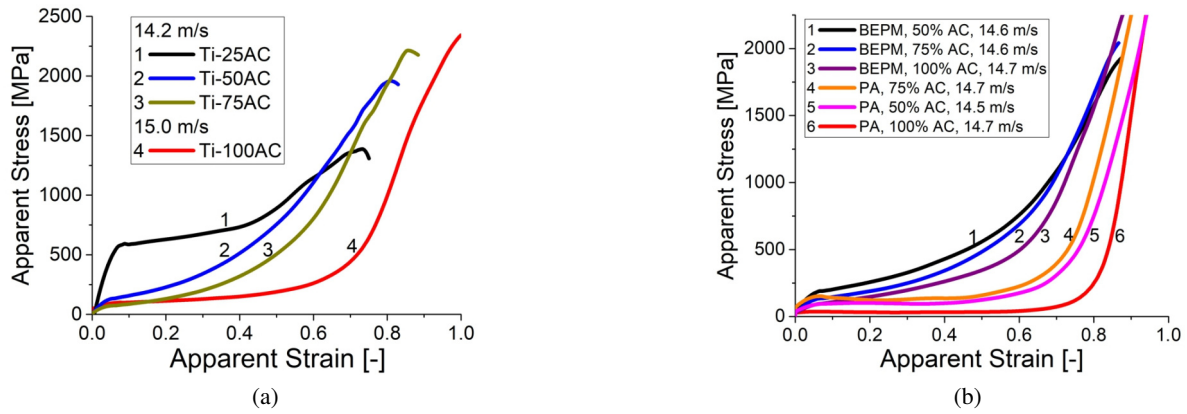
Fig. 6. Dynamic apparent stress-strain curves of the porous samples produced using various AC amounts: (a) porous c.p.Ti (curves 1–3 in (a) are taken from previous work [12], curve 4 present study), and (b) porous Ti-6-4 alloy prepared via BEPM (curves 1–3), or PA (curves 4–6) approaches
