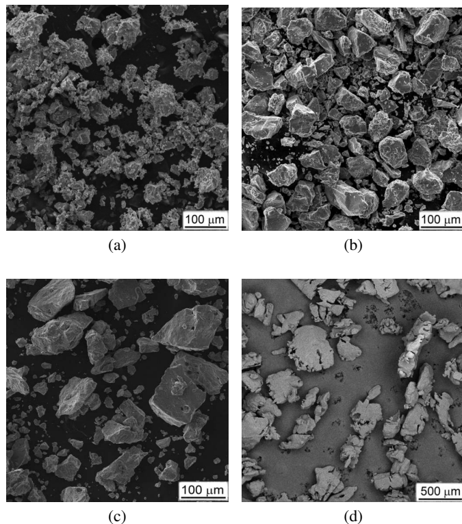
Fig. 1. Powders used for preparation of porous Ti-6-4 materials: (a) TiH_2 , (b) V-Al master alloy, (c) pre-alloyed Ti-6-4 powder, (d) ammonium carbonate. SEM, (a, b) SE, (c) BSE
