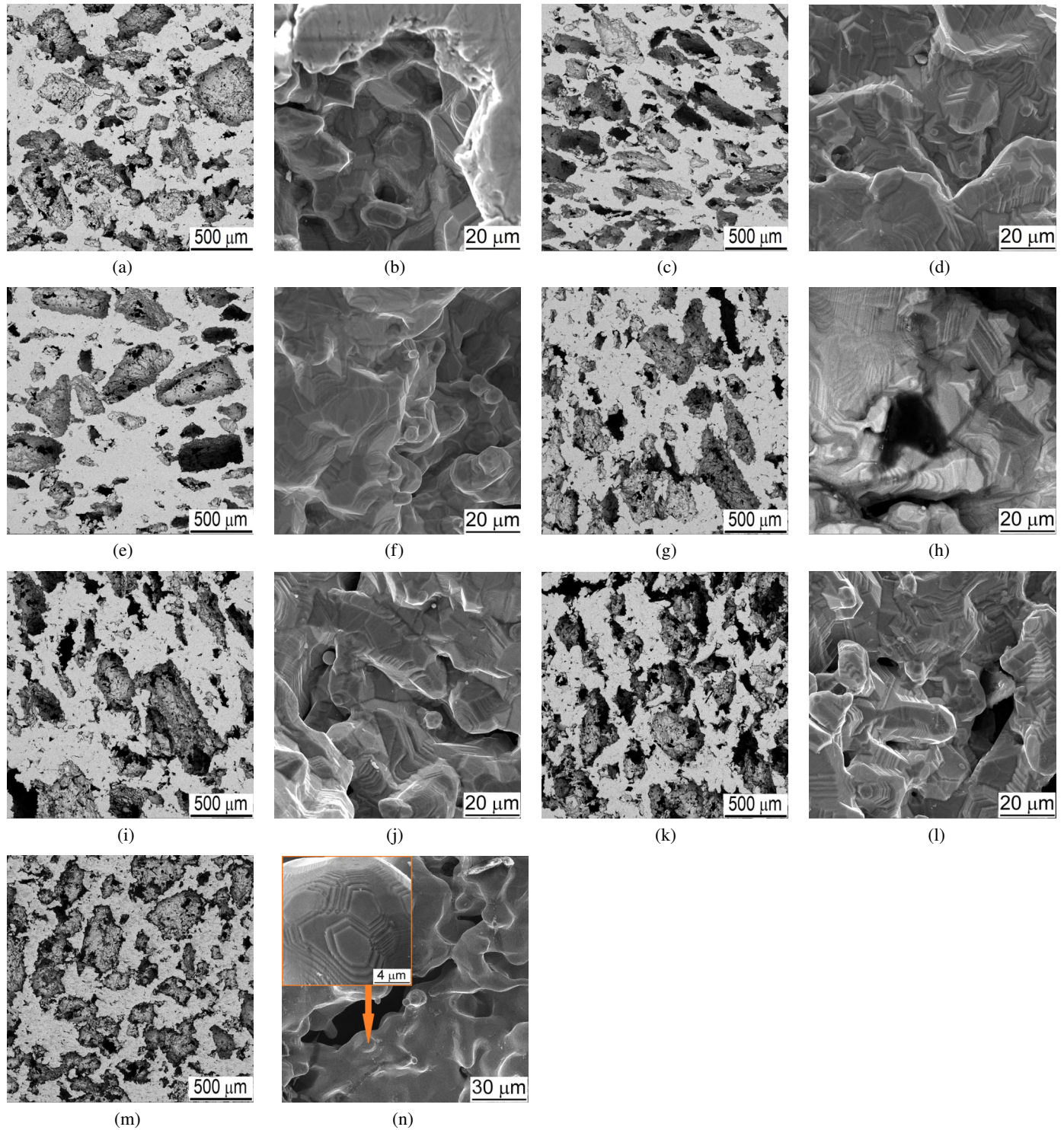
Fig. 3. Microstructure of sintered samples prepared via (a-f) BEPM method, and (g-l) using pre-alloyed powder in the initial (sintered) state. Content of AC: (a, b, g, h) 50%, (c, d, i, j) 75%, (e, f, k, l) 100%; (m, n) Ti100AC. SEM, (a, c, e, g, i, k, m) – side views, BSE; (b, d, f, h, j, l, n) – inner structure of pores, SE
