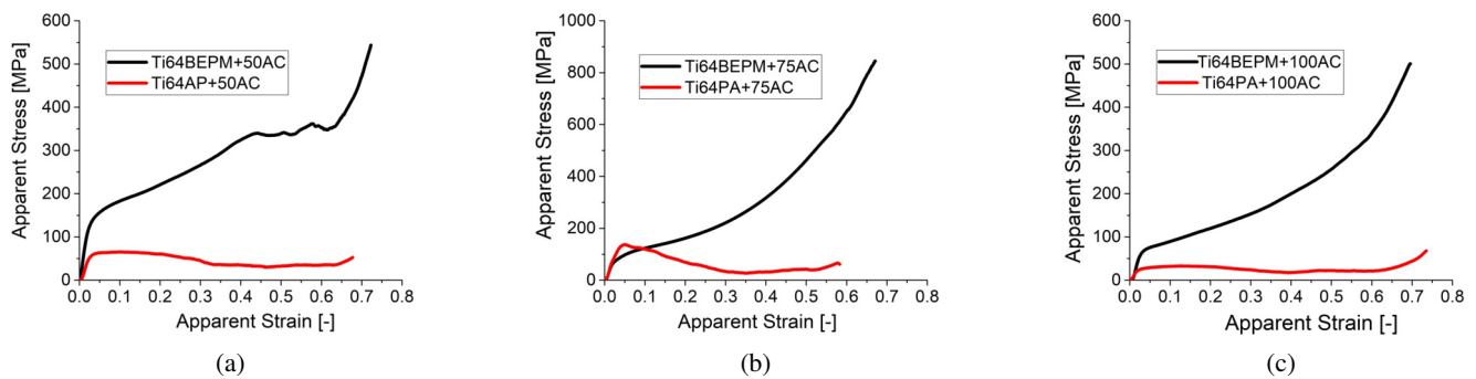
Fig. 8. Apparent stress-strain curves for quasi-static compression tests (strain rate 10^{-3} \text{ s}^{-1} ) of porous Ti64 prepared with AP and BEPM approaches and addition of: (a) 50% AC, (b) 75% AC, and (c) 100% AC
