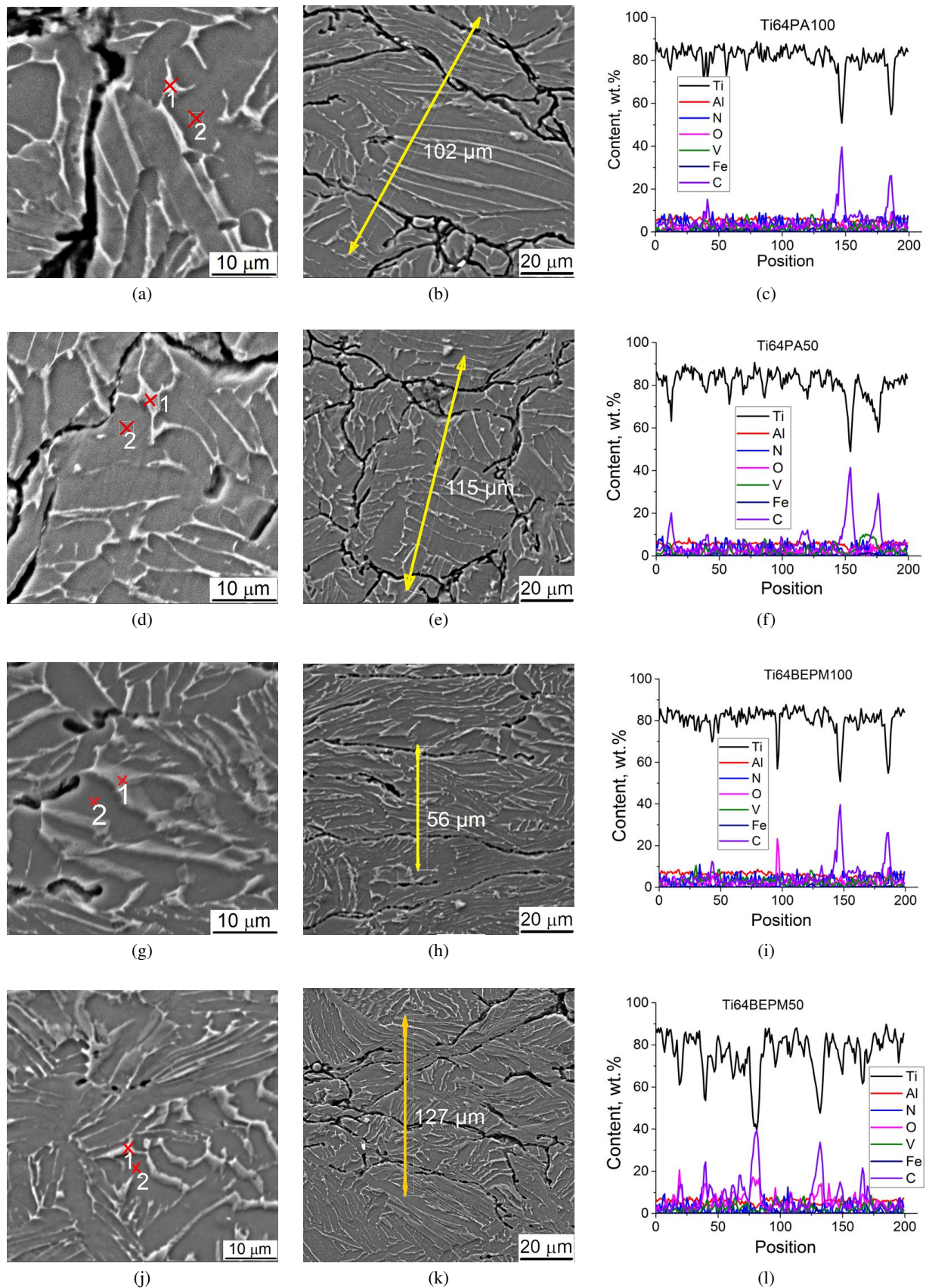
Fig. 14. Images (a, b, d, e, g, h, j, k) SEM, and chemical elements distributions in the samples (a–c) Ti64PA100, (d–f) Ti64PA50, (g–i) Ti64BEPM100, (j–l) Ti64BEPM50 after compression test. Points in (a, d, g, and j) correspond with locations where local chemical analysis was made (see Table 3). Lines in (b, e, h, and k) indicate positions, where distributions of elements were measured (c, f, i, and l)
