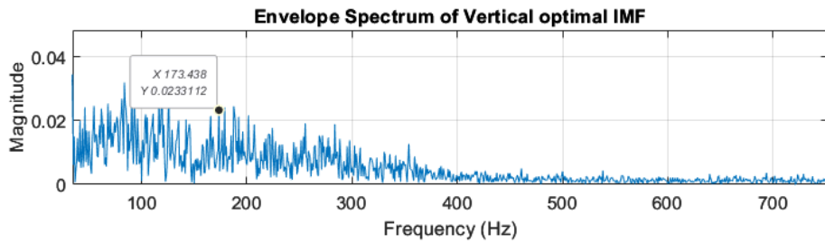
Fig. 22. Envelope spectrum of vertical IMF7
