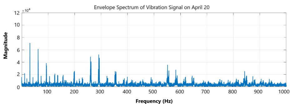
Fig. 26. Envelope power spectrum of the original signal
