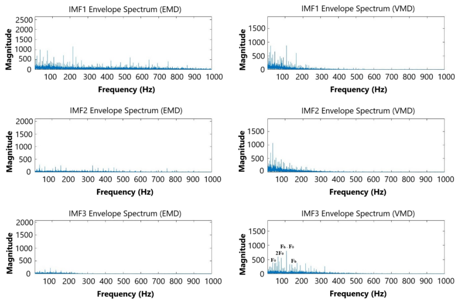
Fig. 15. Envelope spectrum of IMF1-IMF3 after EMD and VMD
