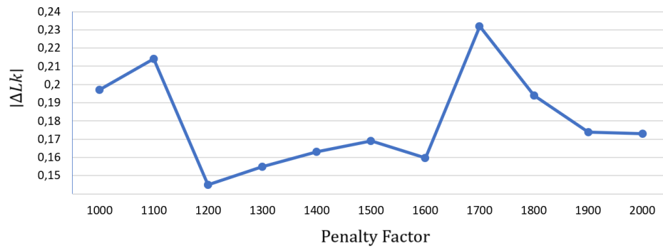
Fig. 18. Change in |\Delta L_k| as a function of Alpha for horizontal signal
