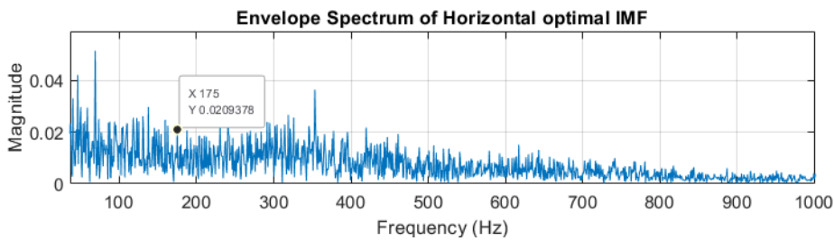
Fig. 23. Envelope spectrum of horizontal IMF3
