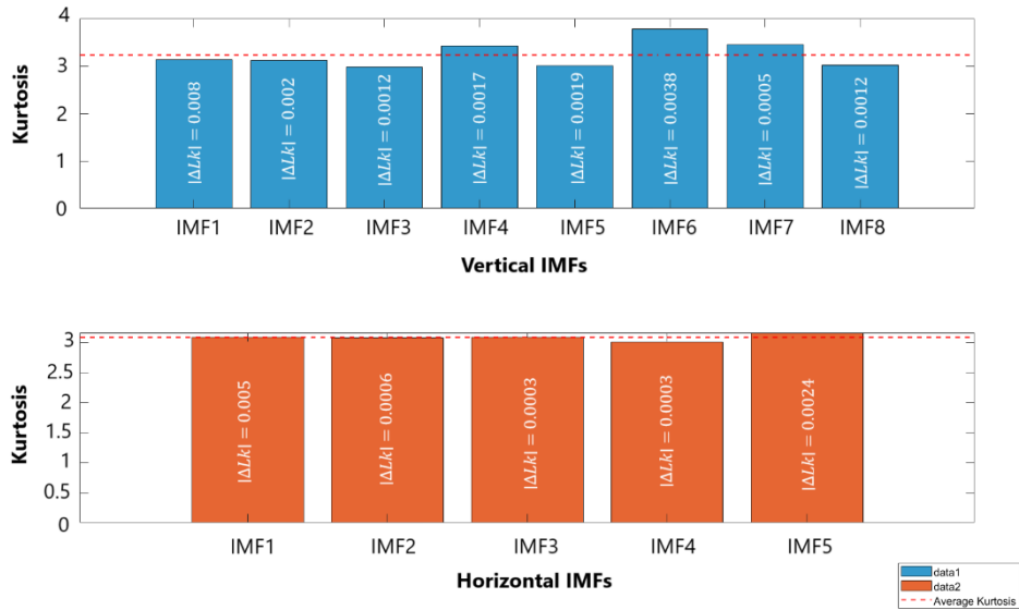
Fig. 21. Kurtosis and |\Delta Lk| for each IMFs (vertical and horizontal signals)
