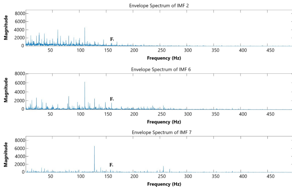
Fig. 7. Envelope spectra of IMF2, IMF6 and IMF7
