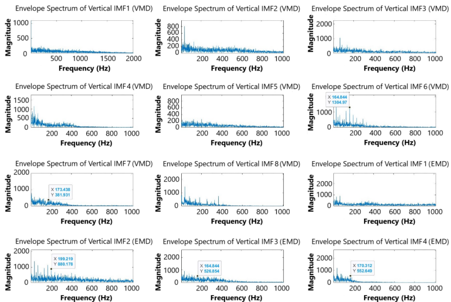
Fig. 25. Comparative envelope analysis of VMD and EMD IMFs for the vertical signal
