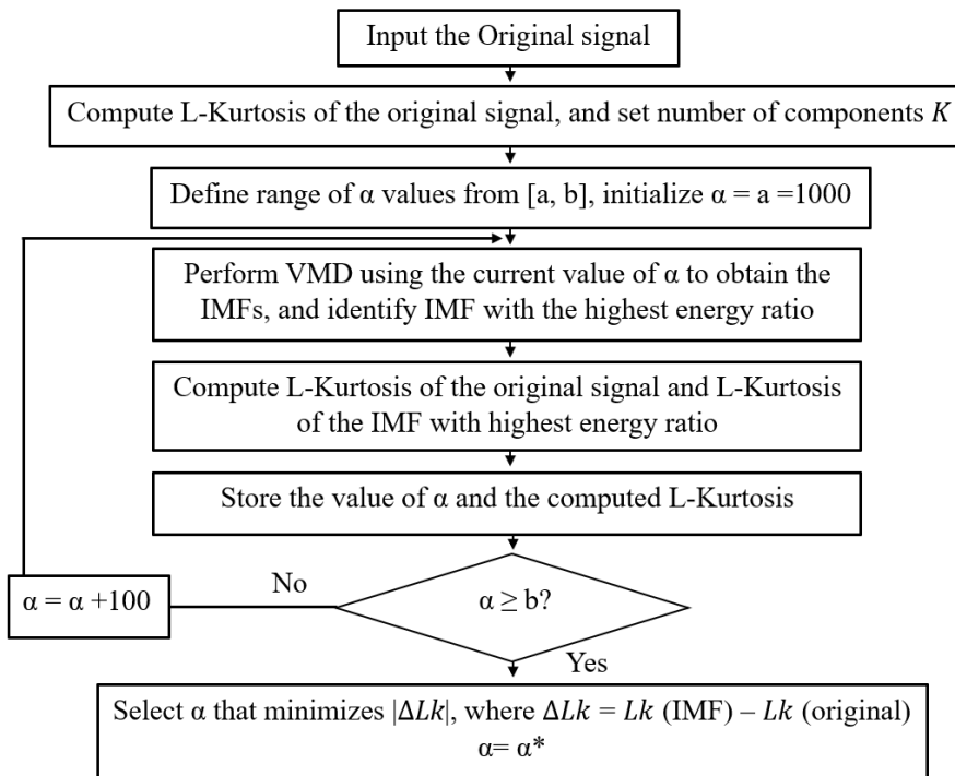
Fig. 1. The proposed algorithm of alpha optimization
