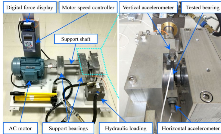
Fig. 16. Experimental Setup of the XJTU-SY Bearing Test Bed [23]
