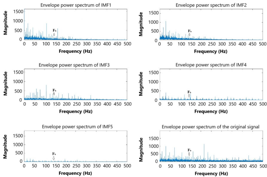
Fig. 13. Frequency domain analysis
