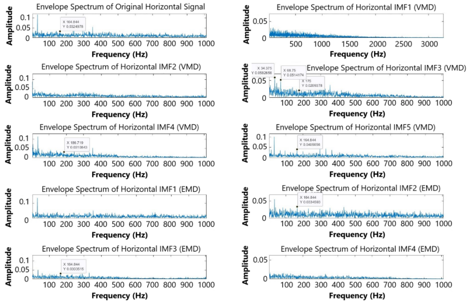
Fig. 24. Comparative envelope analysis of VMD and EMD IMFs for the horizontal signal
