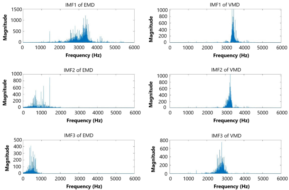
Fig. 14. Spectrum of IMF1-IMF3 after EMD and VMD
