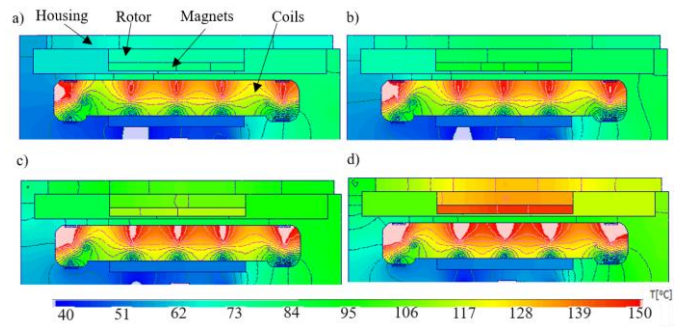
Fig.4. Temperature distribution in the elements of the electromagnetic circuit for the analyzed variants of the rotor: a) A4C0, b) A4C2, c) A2C0, d) A0C0
