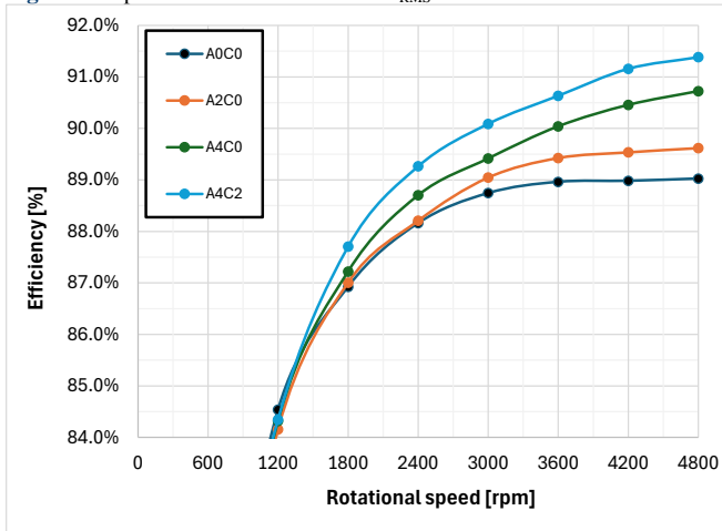
Fig.10. Motor efficiency for rated current I_{RMS} = 240 A
