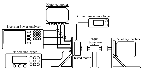
Fig.7. Measurement system of the analyzed motor
