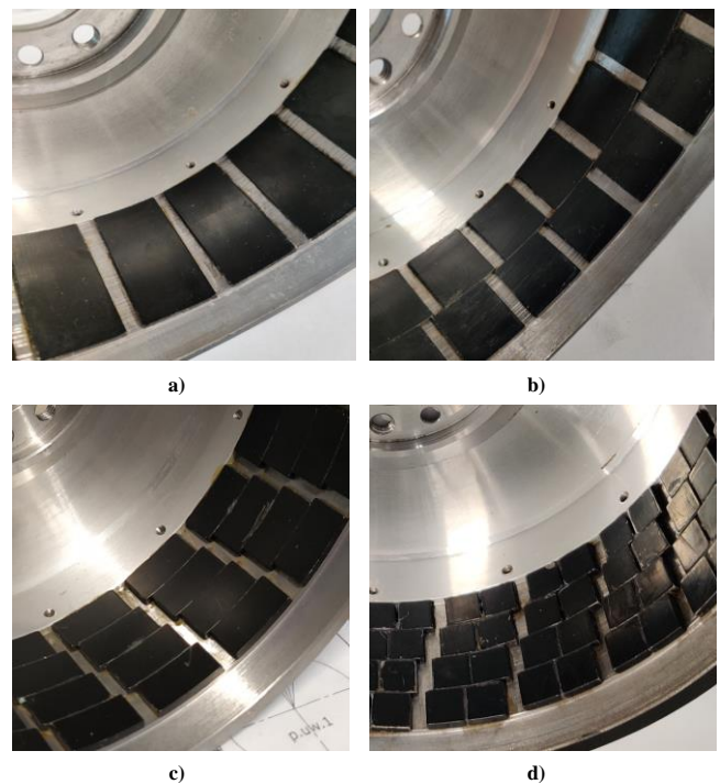
Fig.2. Experimental models of rotors analyzed in this work: a) A0C0, b) A2C0, c) A4C0, d) A4C2
