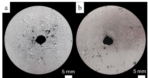
Fig. 7. Macrostructure for the Zn – 2% Bi samples, a) Zn – 2% Bi – without the presence of ultrasonic vibrations, b) Zn – 2% Bi with the presence of ultrasonic vibrations.
