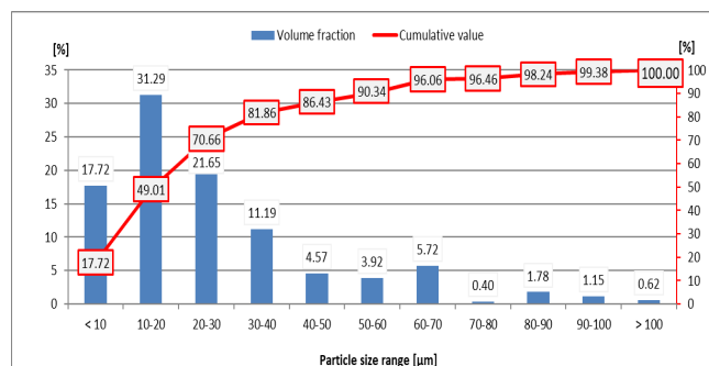
Fig. 3. The particle size distribution of fume deriving from arc welding of 1.4828 steel [23]
