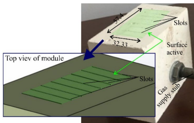
Fig. 3. View of the slot-type module (KS diffusor)
