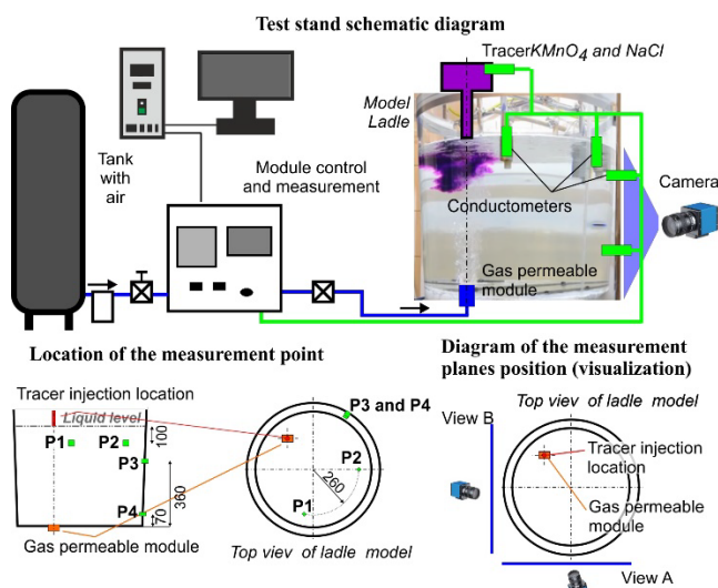
Fig. 2. Test stand schematic diagram (water model ladle)
