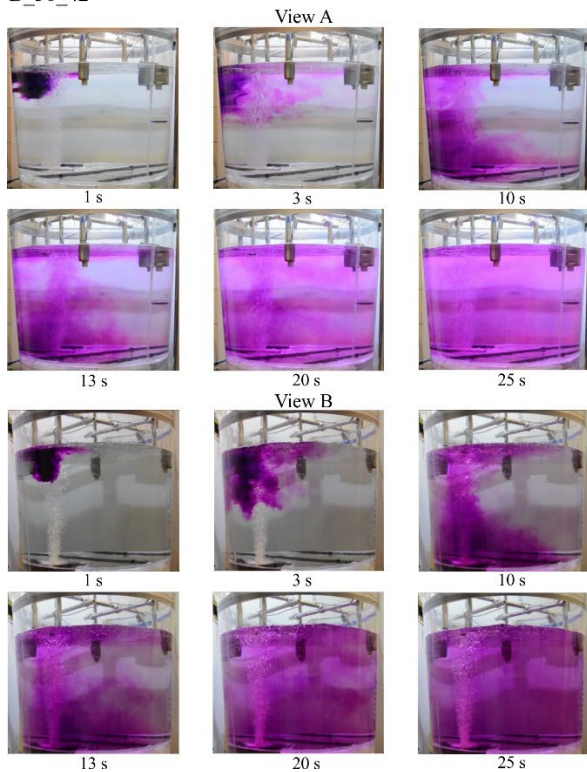
Fig. 6. Visualization of mixing in KS diffuser – type B depending on the experiment variant
