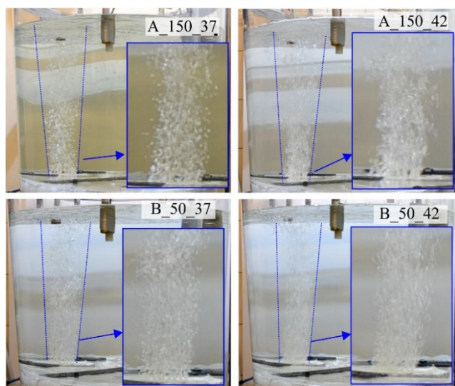
Fig.4. The mechanism of formation of a cone of gas bubbles (gas column) and their degree of dispersion in the model liquid for the considered test variants
