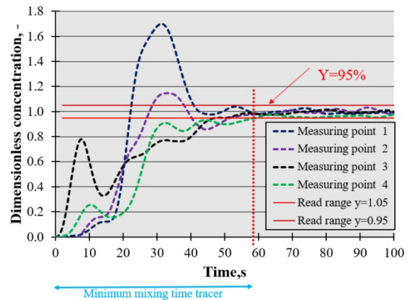
Fig. 7. Water model of mixing-time characteristics – variant B_50_37
