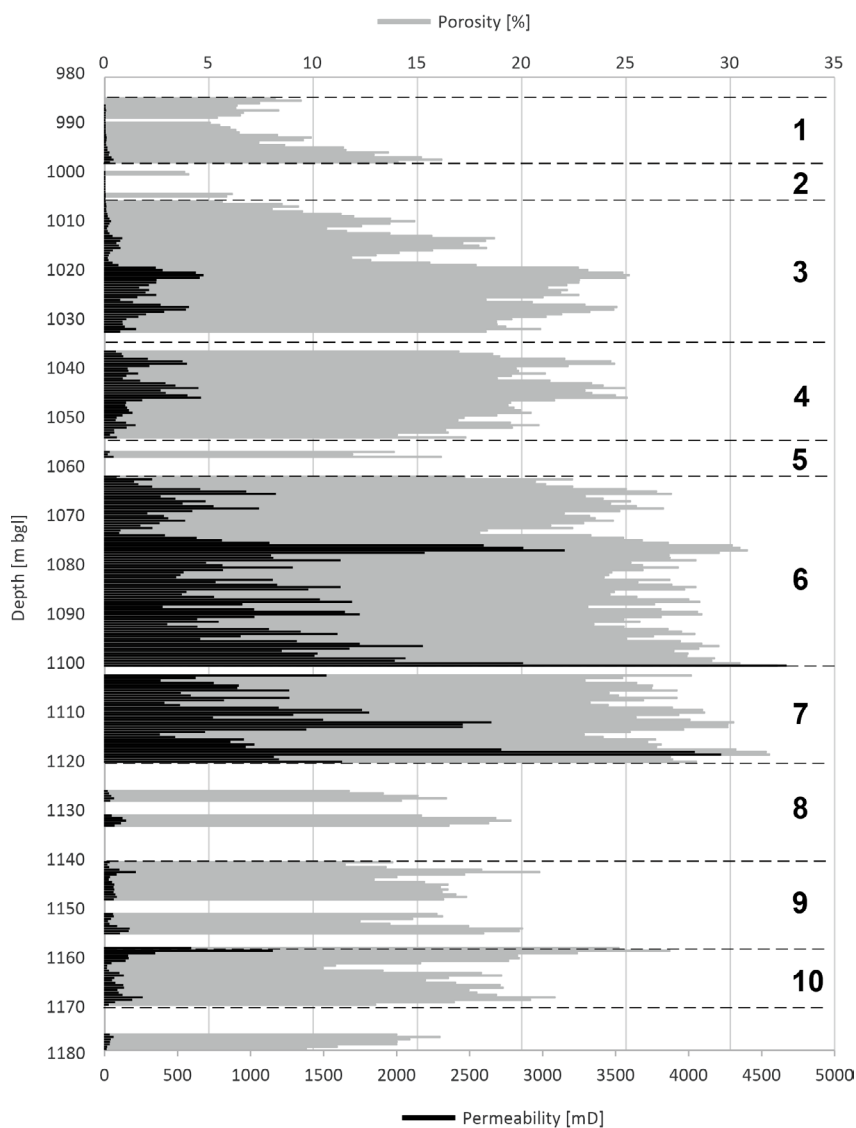
Fig. 4. Porosity and permeability profile of the reservoir in Drzewica Formation in the Jeżów IG-1 well (based on: Wójcicki 2012a)
