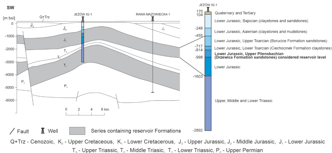
Fig. 1. Geological cross-section through the Jeżów anticline (salt pillow) (based on: Tarkowski 2010)
