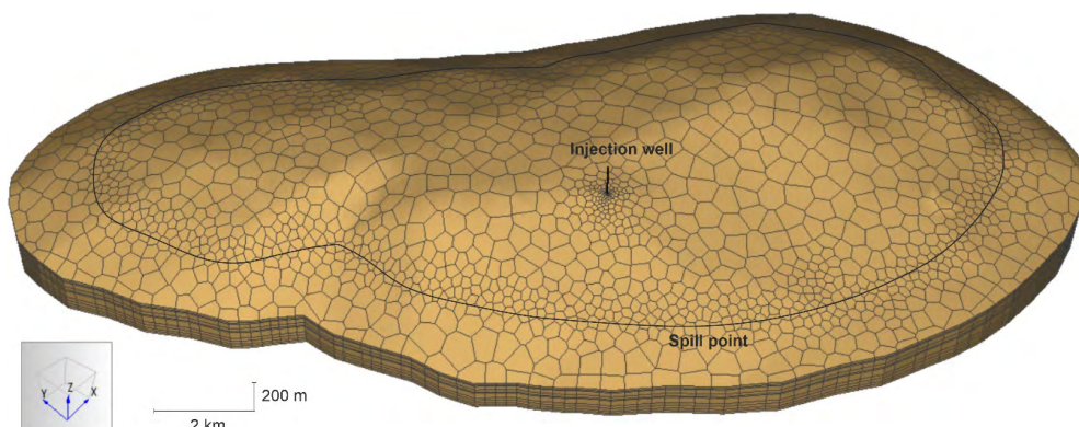
Fig. 3. The model of the Jeżów structure presented in the PetraSim software
