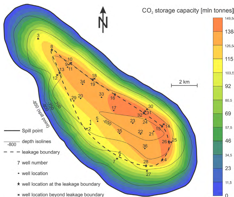
Fig. 5. Map of CO 2 capacity in the Jeżów structure obtained based on capacities collected in the marked and tested injection well locations
