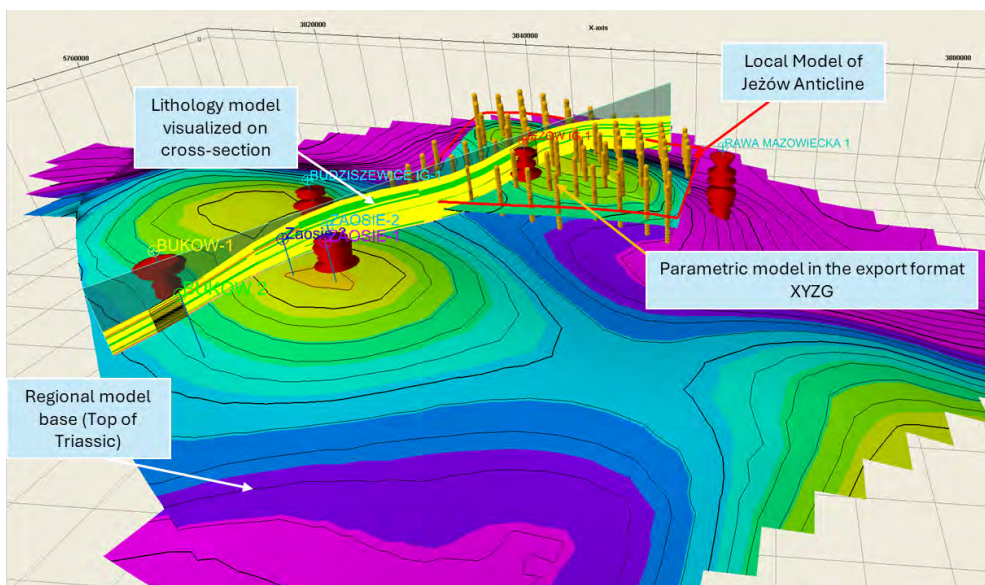
Fig. 2. Regional (Budziszewice–Jeżów) and Local (Jeżów) structural models visualized together with examples of parametric modeling and its export products
