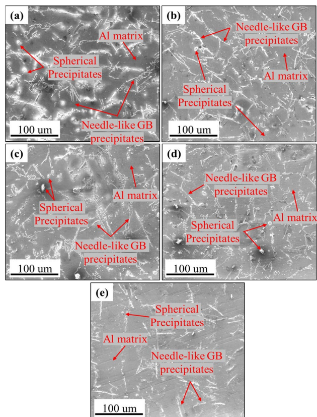
Fig. 7. SEM images of a casted LM-13 Al-alloy sample in molds made from different sand types, showing the morphology of precipitates in the Al matrix: (a) MB sand, (b) HBR sand, (c) SWB sand, (d) MPB sand, and (e) SPB sand. The images highlight the variation in precipitate distribution and morphology within the aluminum matrix
