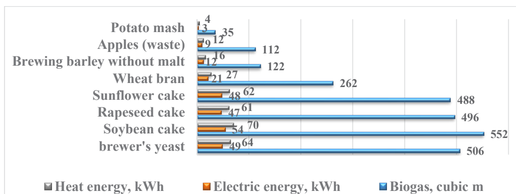
Fig. 5. The amount of energy from 1 ton of processing plant products Source: formed by the authors ( https://biteco-energy.com/ua/biogas-calculator/ )
