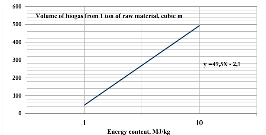
Fig. 4. Dependence of the amount of biogas production on the energy value of plant bioresources
