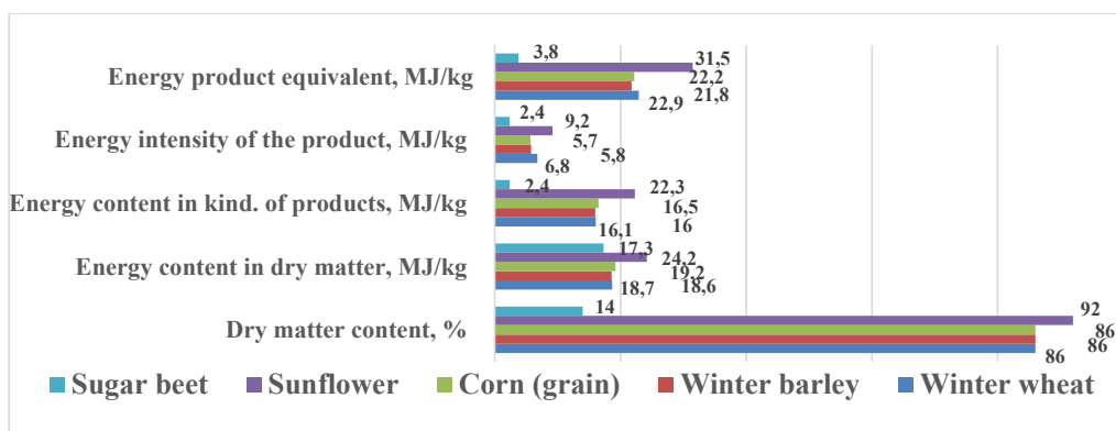
Fig. 3. Energy equivalents of crop production
