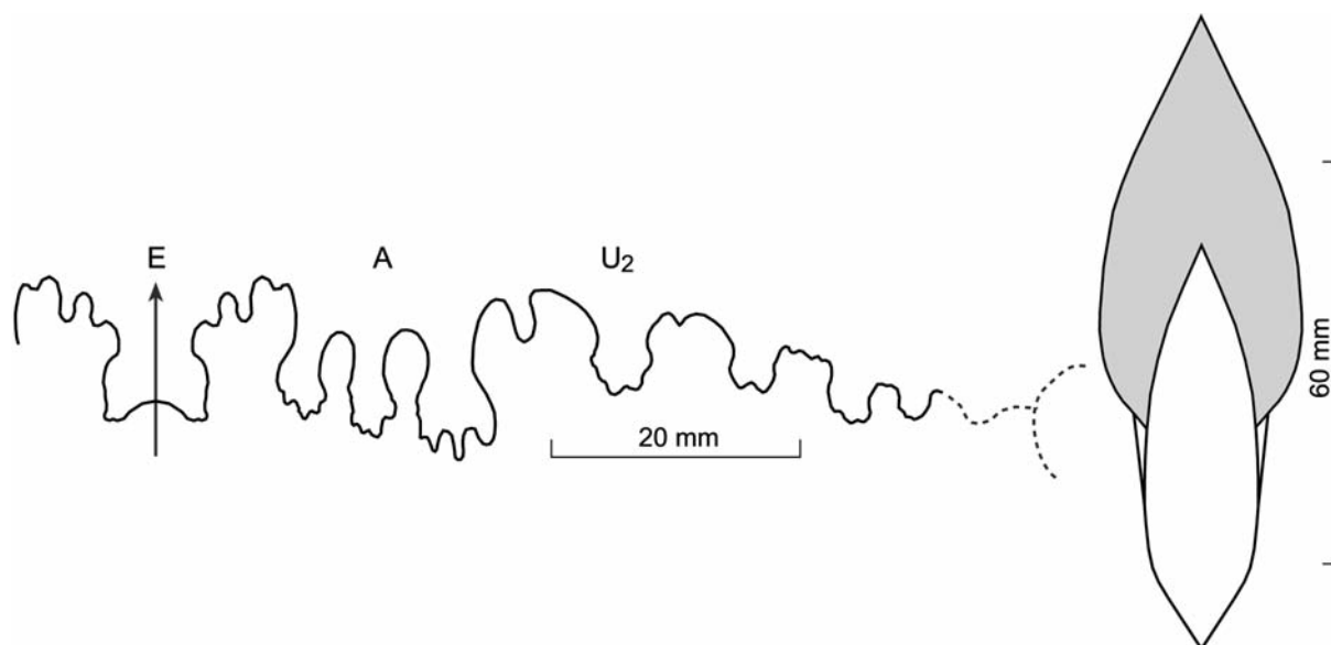
Text-fig. 20. Suture line and whorl section of Coilopoceras requienianum (d'Orbigny, 1841), Upper Turonian of the Umm Omeiyid Formation, specimen AfK 339
