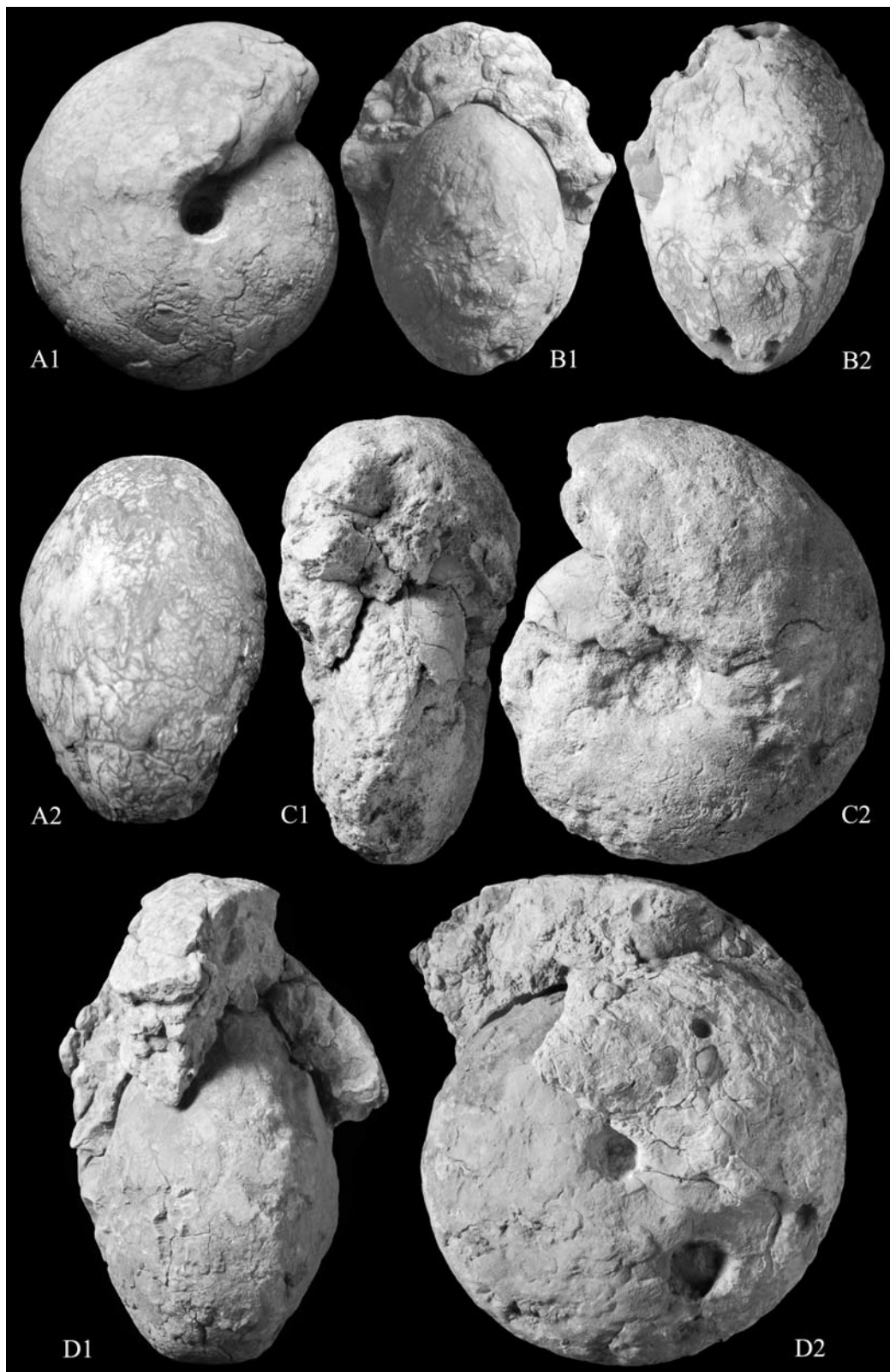
Text-fig. 13. A – Vasoceras kossmati Choffât, 1898 (A1, A2 – lateral and ventral views of AfK 311, \times 1 ). B – Neoptychites cephalotus (Courtillet, 1860) (B1, B2 – apertural and ventral views of AfK 313, \times 1 ). C – Thomasites gongilensis (Woods, 1911) (C1, C2 – apertural and lateral views of AfK 314, \times 1 ). D – Thomasites rollandi (Thomas and Peron, 1889) (D1, D2 – apertural and lateral views of AfK 316, \times 1 ). All specimens from the Lower Turonian of the Galala Formation
