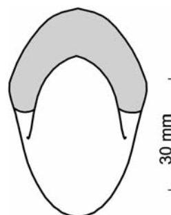
Text-fig. 11. Whorl section of Neptychites cephalotus (Courtillet, 1860), Lower Turonian of the Galala Formation, specimen AfK 313
