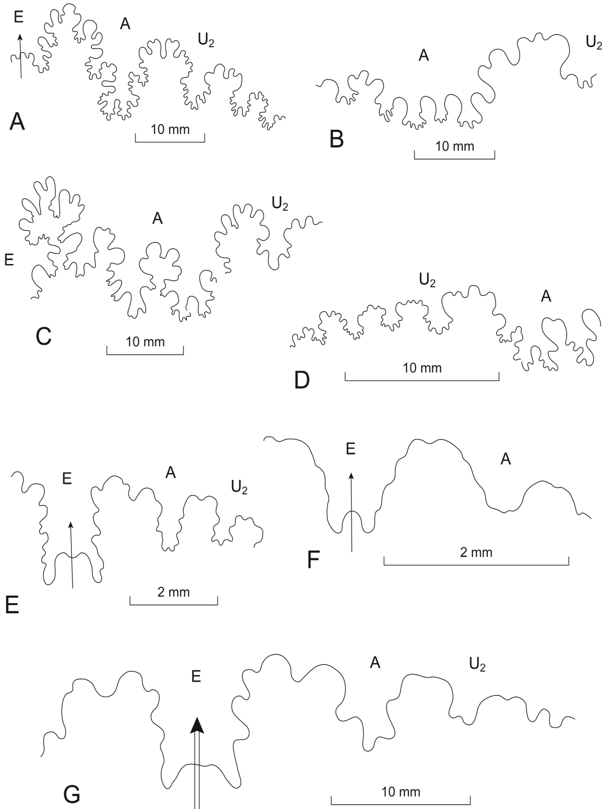
Text-fig. 20. Suture lines. A – Neptychites cephalotus (Courtyllier, 1860), UM Sen010a. B – Wrightoceras wallsi Reyment, 1954, FSIT FR3. C, D – Coilopoceras springeri Hyatt, 1903. C, REII; D, FSIT MS6. E, G – Romaniceras sp. juv. E – FSIT CTP2; G – FSIT MN5P5. F – Vascoceras sp. juv., FSIT MSSP6.
