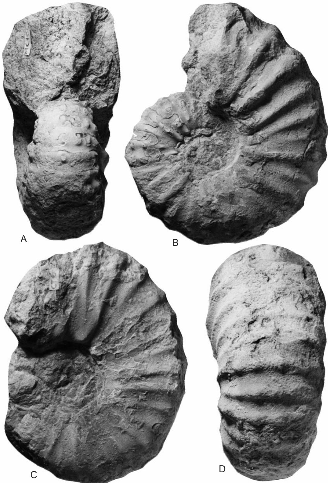
Text-fig. 18. A, B – Romaniceras (Yubariceras) ornatissimum (Stoliczka, 1865), FSIT MC15, from the Calcaires de Montplaisir (Saint-Louis syncline). C, D – Romaniceras (Romaniceras) mexicanum Jones, 1938, FSIT CT6, from Les Capitaines. All figures are \times 1
