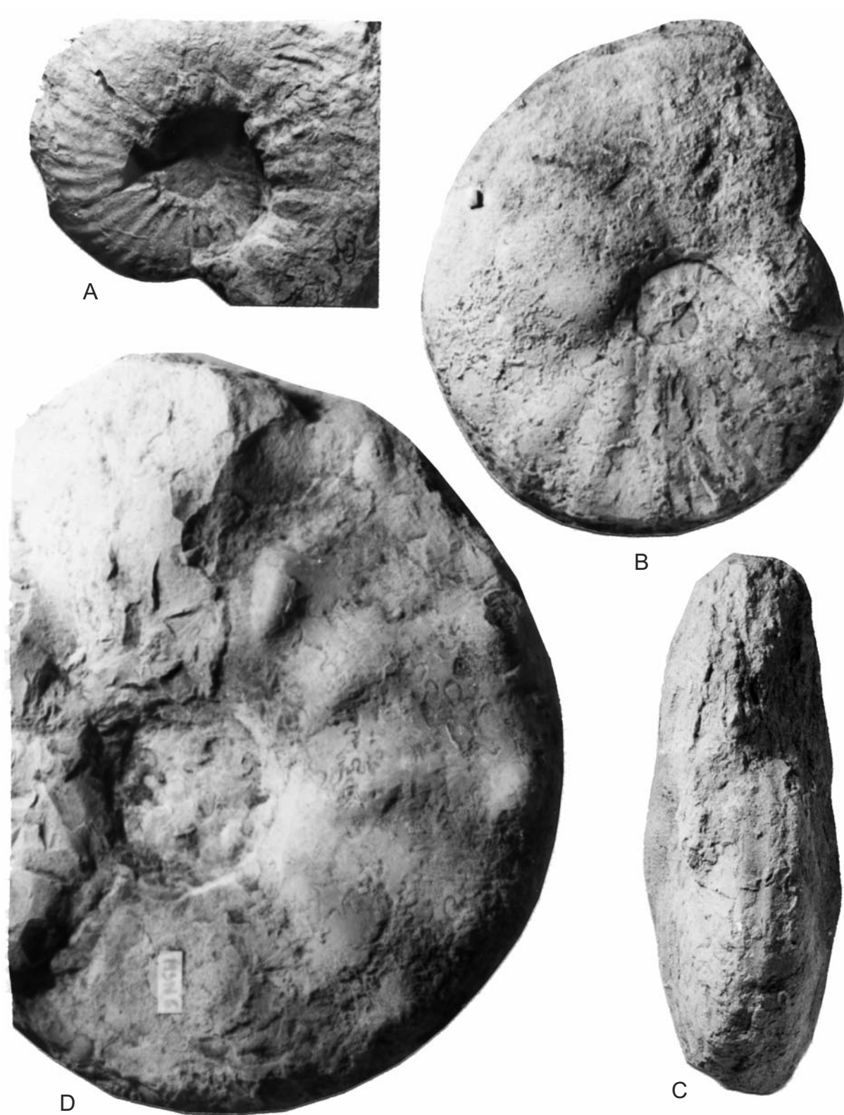
Text-fig. 19. A – Romaniceras (Romaniceras) mexicanum Jones, 1938, FSIT MS3, from NW of Marsa (Padern area). B, C – Pseudotissotia galliennei (d’Orbigny, 1850), FSIT MC5, from the Calcaires de Montplaisir (Saint-Louis syncline). D – Mammites nodosoides (Schlüter, 1871), FSIT MSN5a, from NE of Marsa. All figures are \times 1
