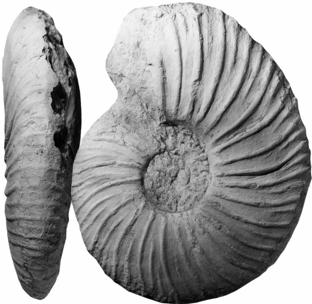
Text-fig. 13. Pachdesmoceras linderi (de Grossouvre, 1894), the lectotype, MNHP R51861, the original of de Grossouvre, 1894, pl. 18, from the environs of Padern. The figure is reduced \times 0.8 approximately
