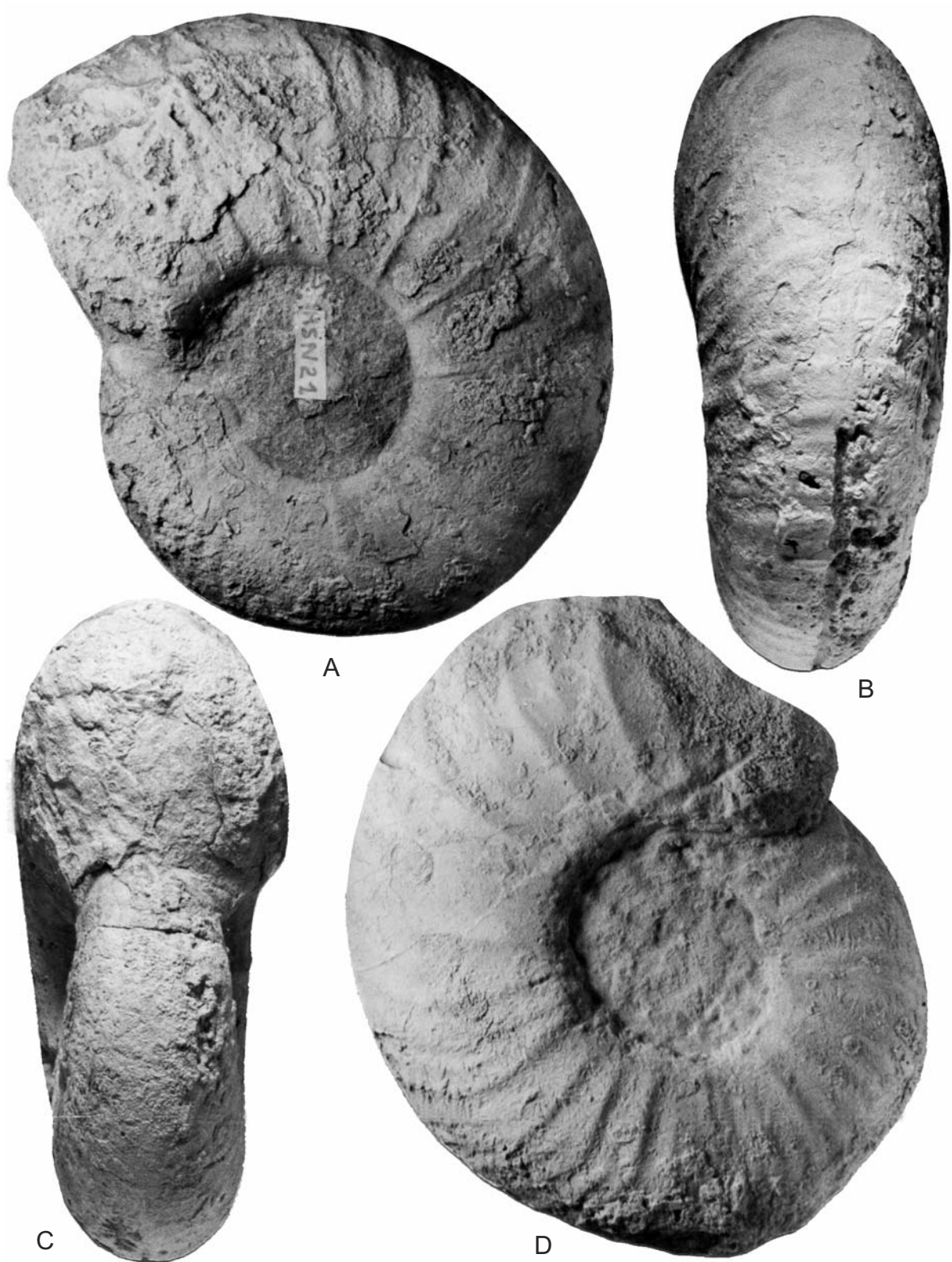
Text-fig. 11. Pachydesmoceras kossmati Matsumoto, 1987. A, B – FSIT MSN21, from NE of Marsa (Padem area); C, D – FSIT M9, from Baillesats. All figures are \times 1
