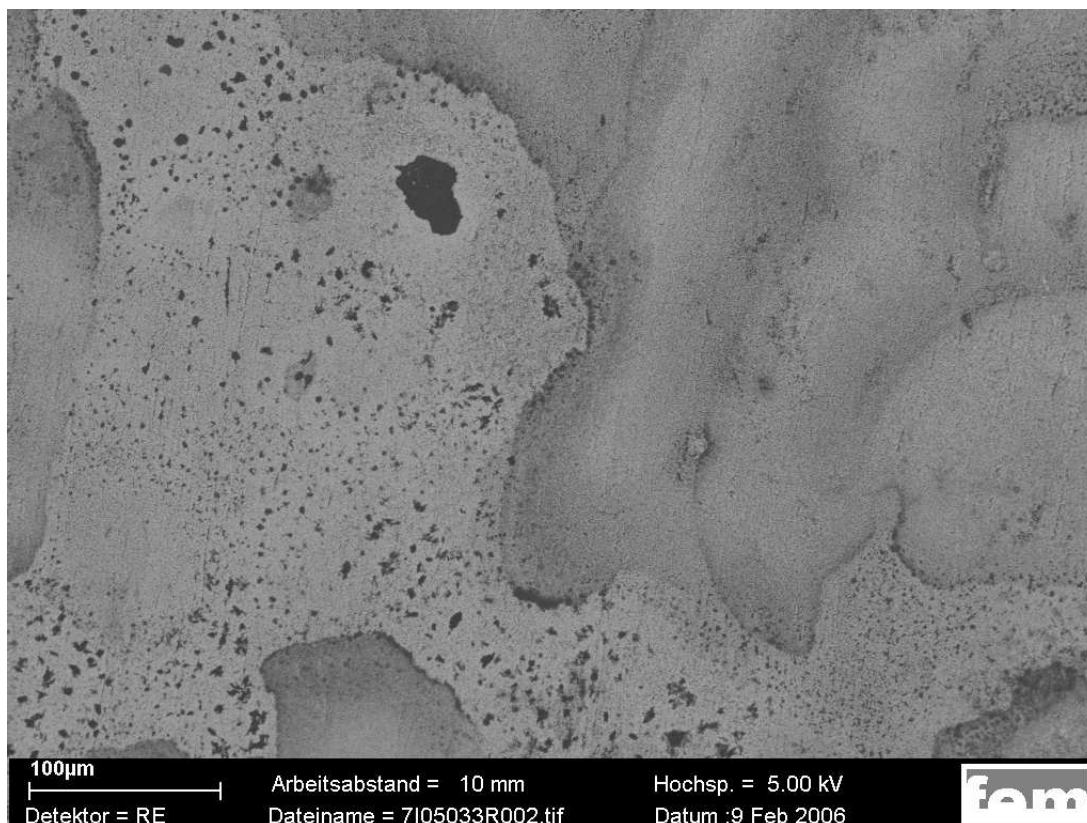
Fig. 3b. SEM image of a small area of the coating from Figure 3a
