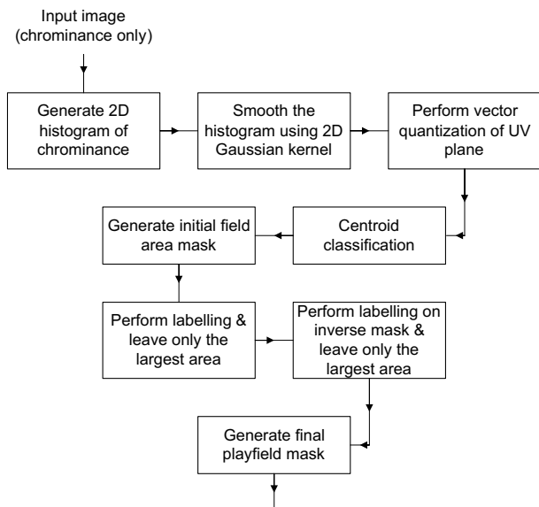
Fig. 2. Playfield detection algorithm flow diagram.
