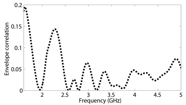
Fig. 14. Calculated envelope correlation coefficient from S-parameters.
