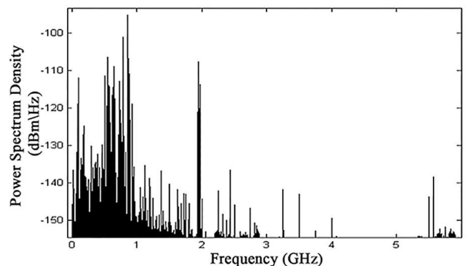
Fig. 1. Measurement of 0-6 GHz spectrum utilization [7].
