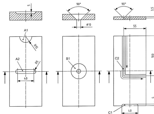
Fig. 10. Dimensions of samples used for padding and welding, simulating the typical casting defects, according to PN EN 15614-4
