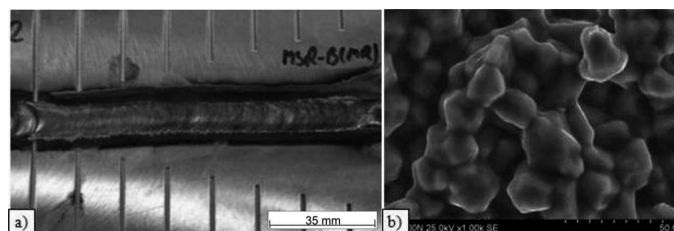
Fig. 6. Houldcroft test results for the QE22 alloy: a) a remelted plate with a visible crack in the weld axis, b) crack area in the weld penetration, SEM
