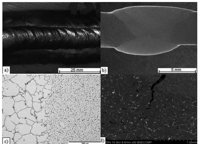
Fig. 9. QE22 alloy joint ( I = 120 A, El = 3.0 kJ/cm): a) weld face, b) macrostructure of two-sided butt joint – correct joint condition, as-cast, c) refinement of microstructure in the weld fusion line, as-cast condition, LM d) hot crack in weld and network of cracks in HAZ, SEM
