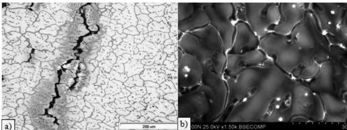
Fig. 8. Penetration microstructure after the Transvarestraint test: a) hot crack on the borders of weld dendrites, LM, b) fracture surface with a visible (\text{Mg,Ag})_{12}\text{Nd} phase in the interdendritic areas, SEM
