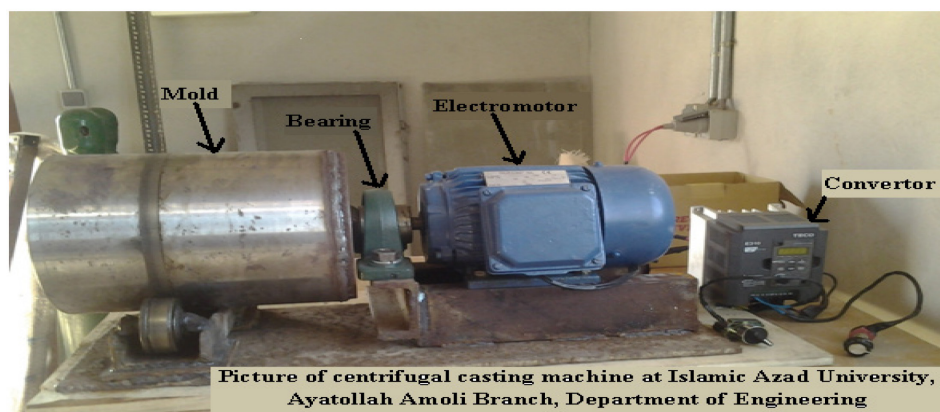
Fig. 3. Components of a centrifugal casting machine
