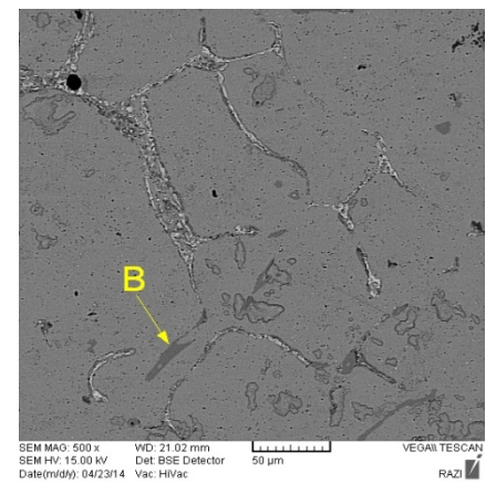
Fig. 8. SEM with EDS of intermetallic \text{Cu}_6\text{Sn}_5 particles (phase of B), Back scattered Electron (BSE), magnification of 500
