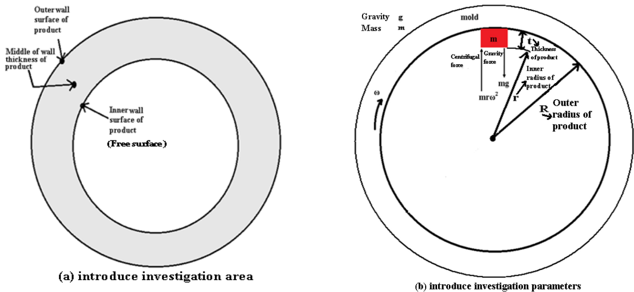
Fig. 2. The horizontal centrifugal casting
