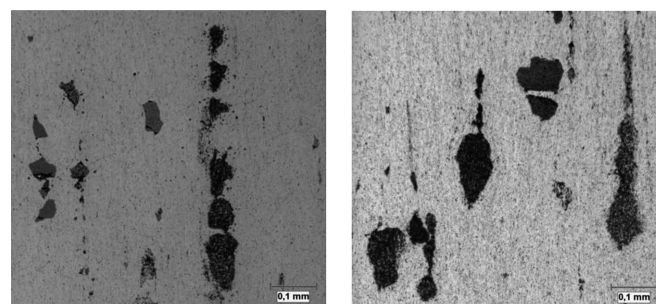
a) Al+2,5%SiC magn. 100x
