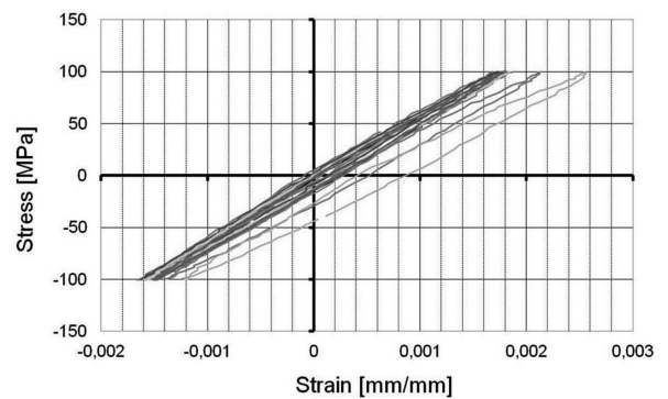
Fig. 10. Hysteresis loops for the cycles over 100 of fatigue tests. Material Al+2,5%SiC (second series) tested at stress amplitude equal to 100 MPa
