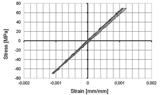
Fig. 8. Hysteresis loops for the cycles over 100 of fatigue tests. Material Al+10%SiC (second series) tested at stress amplitude equal to 70 MPa
