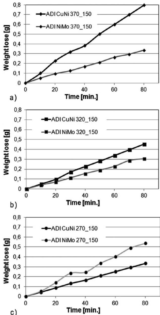
Fig. 6. The results of tests in dry corundum abrasive. Compressive stress: 0.125MPa
