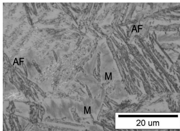
Fig. 15. Ductile iron matrix in a surface layer of ADI NiMo 370_150 sample – ausferrite AF + martensite M
