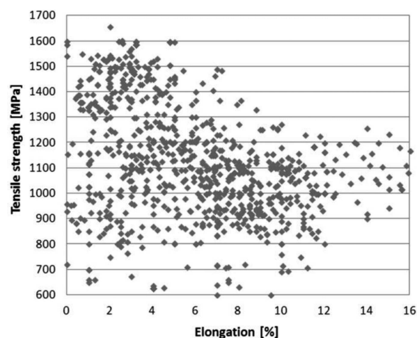
Fig. 1. Austempered ductile iron tensile strength vs elongation
