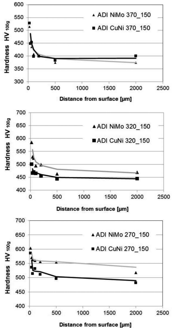
Fig. 9. The results of hardness measurements displayed as a distribution of values in direction from the sample surface: a) ADI_370_150, b) ADI_320_150, c) ADI_270_150
