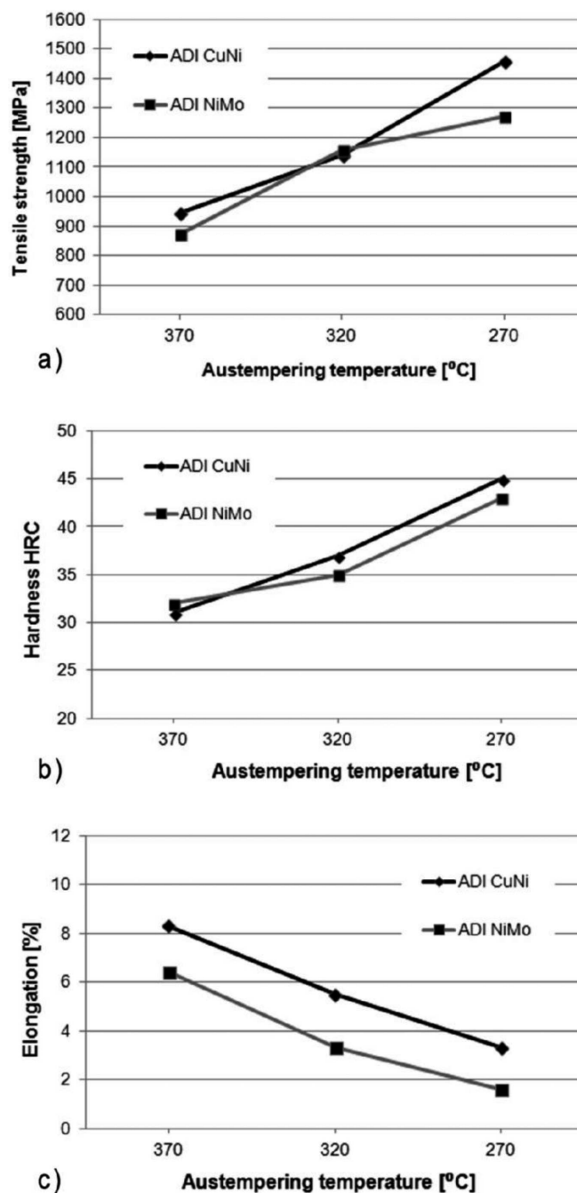
Fig. 4. Graphical display of the results of basic studies of the mechanical properties
