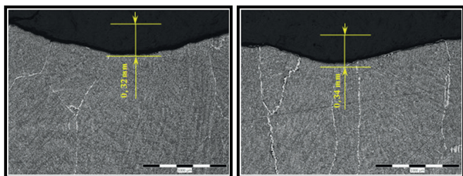
Fig. 6. Microstructure under abnormal oscillation marks observed at short negative strip time and a higher casting speed ( V_c = 2.4 m/min, T_n = 0.088 s, \%T_n = -50 %)
