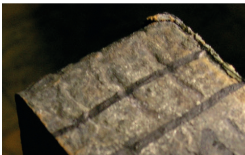
Fig. 5. Abnormal oscillation marks observed in corner areas of billets surface cast with short negative strip time and a higher casting speed ( V_c = 2.4 m/min, T_n = 0.088 s, \%T_n = -50 %)
