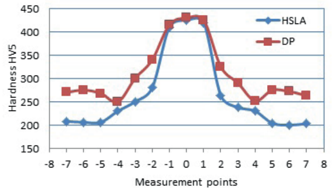
Fig. 18. Hardness distribution on the cross-section of the joint made with the single beam at a welding rate 11 m/min with the entire penetration
