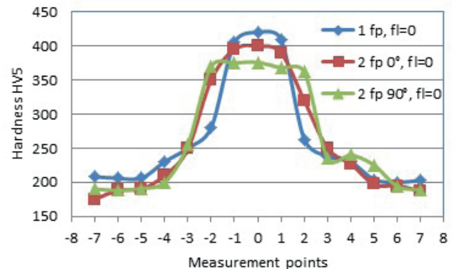
Fig. 19. Joint hardness distribution measured at the half of the HSLA steel sheet thickness for individual positions of laser beam focuses
