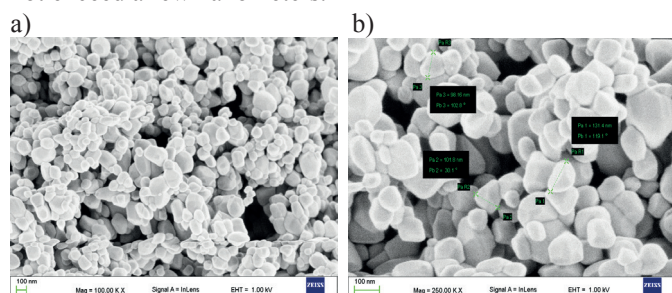
Fig. 6. SEM image of TiO 2 micro powder registered at a magnification: a) 100 kx, b) 250 kx
