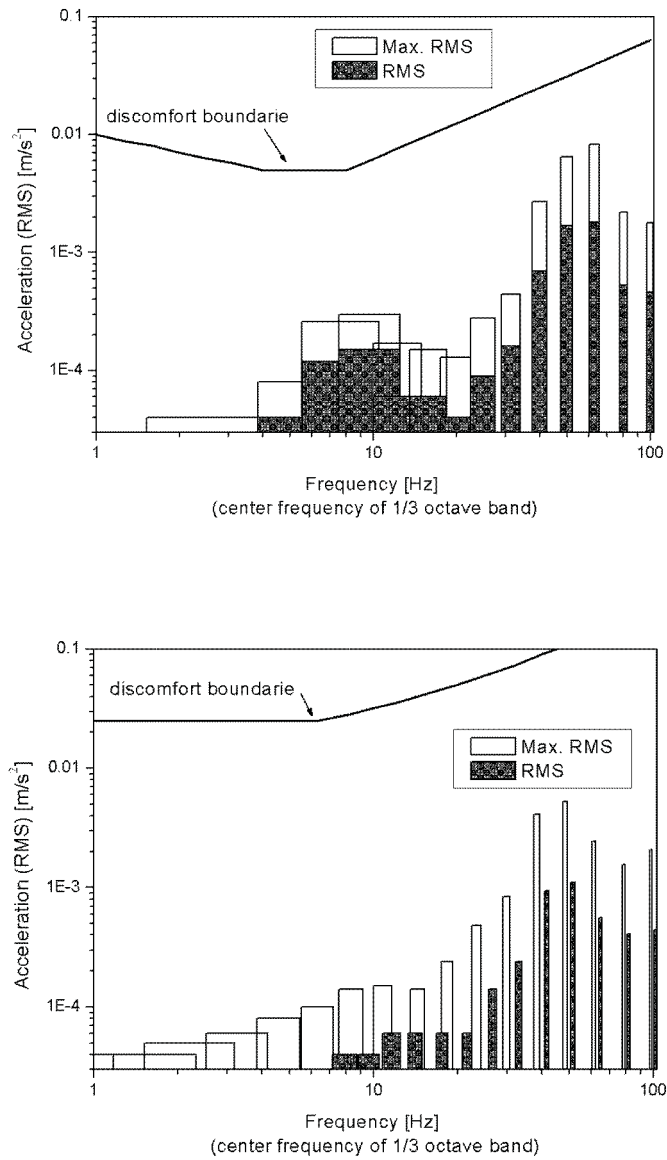
Fig. 20. Diagrams of root mean square and maximum root mean square value of accelerations in vertical (top) and lateral (bottom) direction on the basement in the building near the curved section of the track
