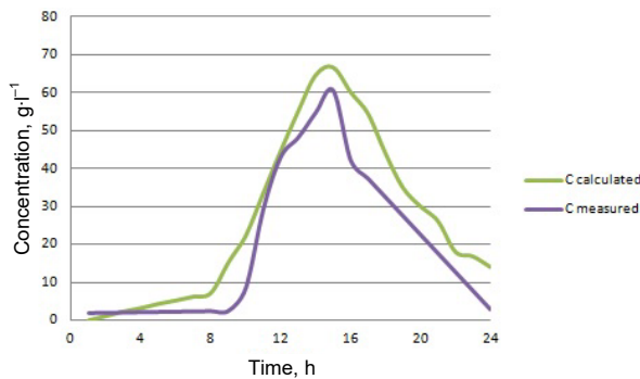
Fig. 8. Event of 6 th March 1986: concentration measured and calculated par HEC-RAS in Chemora station
