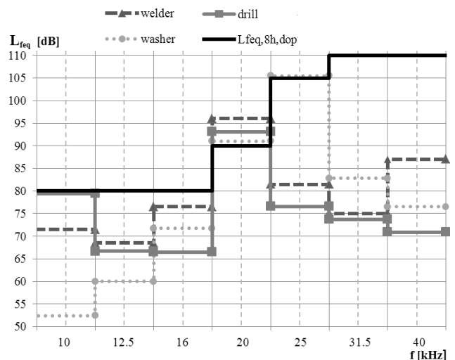
Fig. 1. Measurements results of equivalent sound pressure levels at work stations with: a typical welder, a washer and a drill ( L_{f_{eq},8h,dop} = \text{MAI} ).
