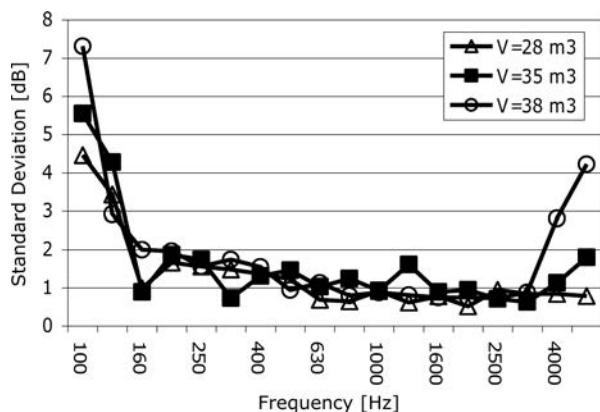
Fig. 7. Standard deviation as function of the frequency for three examples in which a different effect of the wall vibration is observed. The partition volume for each example is specified in the figure.
